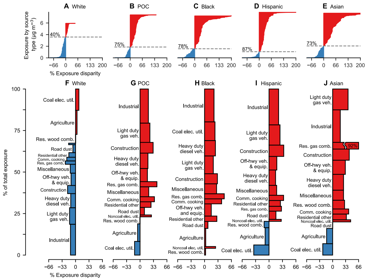
Fig. 1. Source contributions to racial-ethnic disparity in PM_{2.5} exposure. (A to E) Individual source type ( n = 5434 source types) contributions to exposure ( y axis) and % exposure disparity ( x axis, truncated at 200%, positive values are shaded red, negative values are shaded blue), with dashed lines denoting percent exposure caused by sources with positive exposure disparity. (F to J) Sources in (A) to (E) grouped into source sectors ( n = 14 groups) and ranked vertically according to absolute exposure disparity, proportional to the area of each rectangle. As shown in (B), POC experience greater-than-average exposures from source types causing 75% of overall exposure. Source: data file S1, which also includes results for individual states and urban areas.
