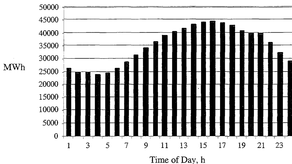
Figure 3.1. Daily electricity load profile in CA on a summer weekday (Aug 8, 2000) (CAISO 2000).
