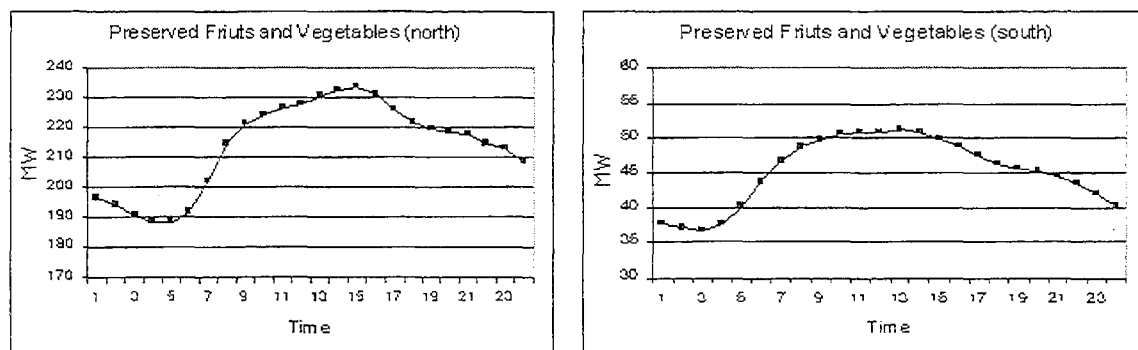
Figure 6.7. Load profiles during a peak day for the preserved fruits and vegetable industry; Northern and Southern California
