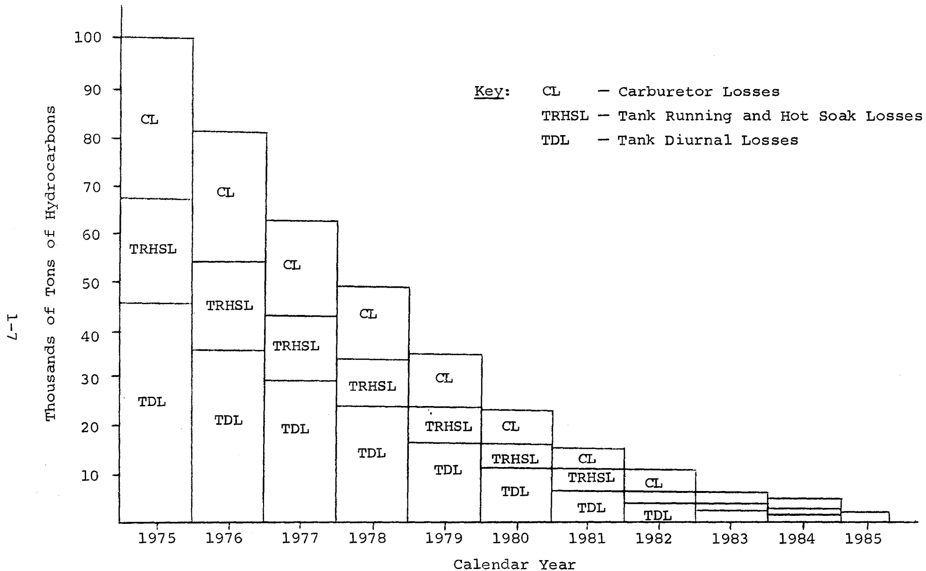
Figure 1-1. EVAPORATIVE EMISSIONS FROM PRE-1970 LIGHT-DUTY VEHICLES BY SOURCE
