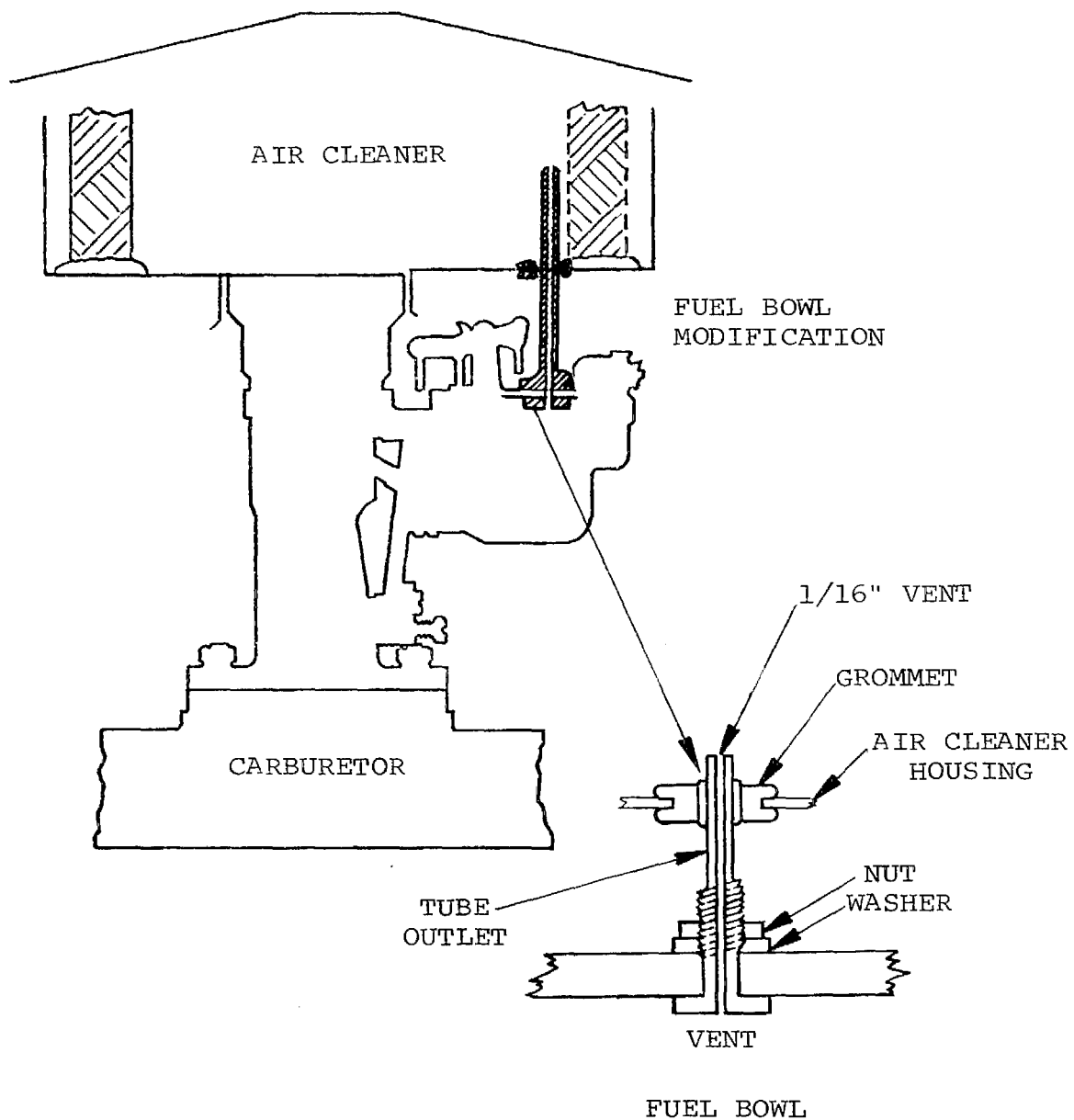
Figure 2-7. FUEL BOWL VENTED TO AIR CLEANER
