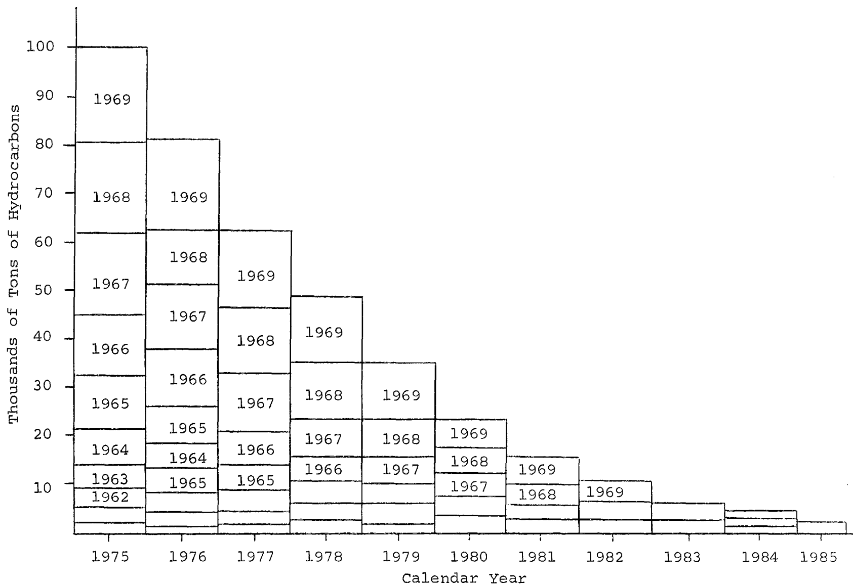
Figure 1-2. EVAPORATIVE EMISSIONS FROM PRE-1970 LIGHT-DUTY VEHICLES BY AGE GROUP
