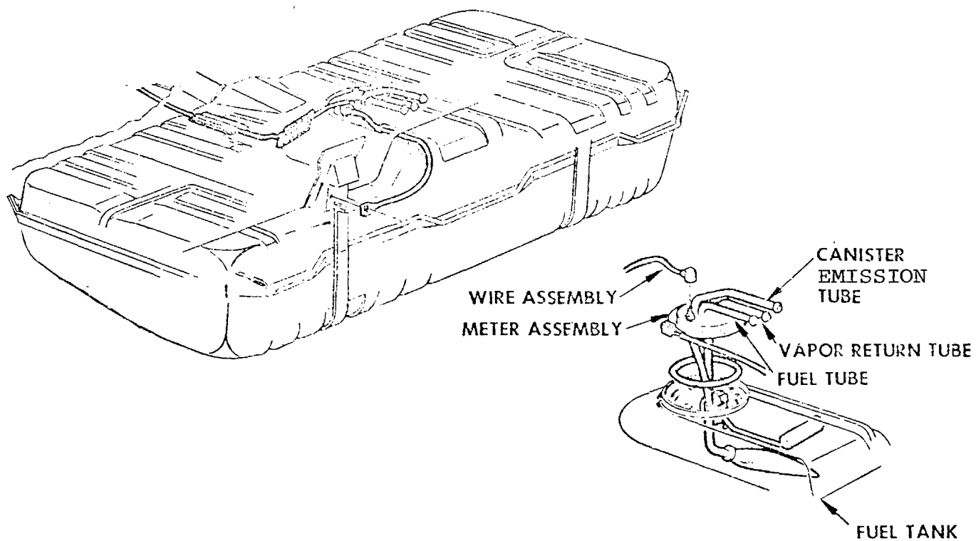
Figure 2-3. VENTED SENDING UNIT MODIFICATION
