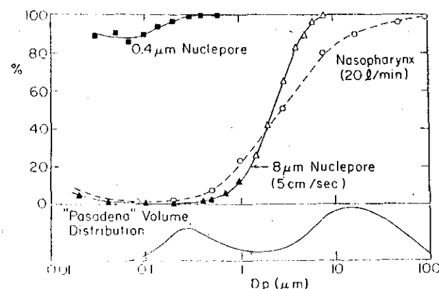
Figure 2. Particle capture efficiencies of 8.0\text{-}\mu\text{m} and 0.4\text{-}\mu\text{m} Nuclepore filters for a face velocity of 5\text{ cm/s} .
