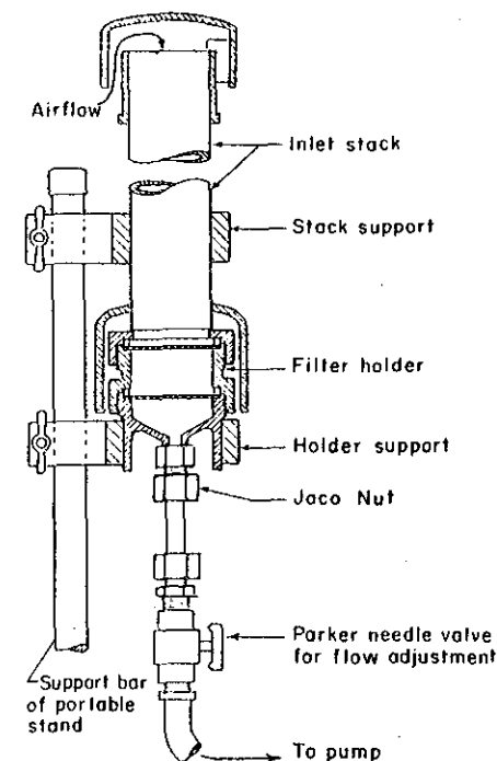
Figure 1. Schematic of the stacked filter unit showing the inlet and the 2-stage filter holder
