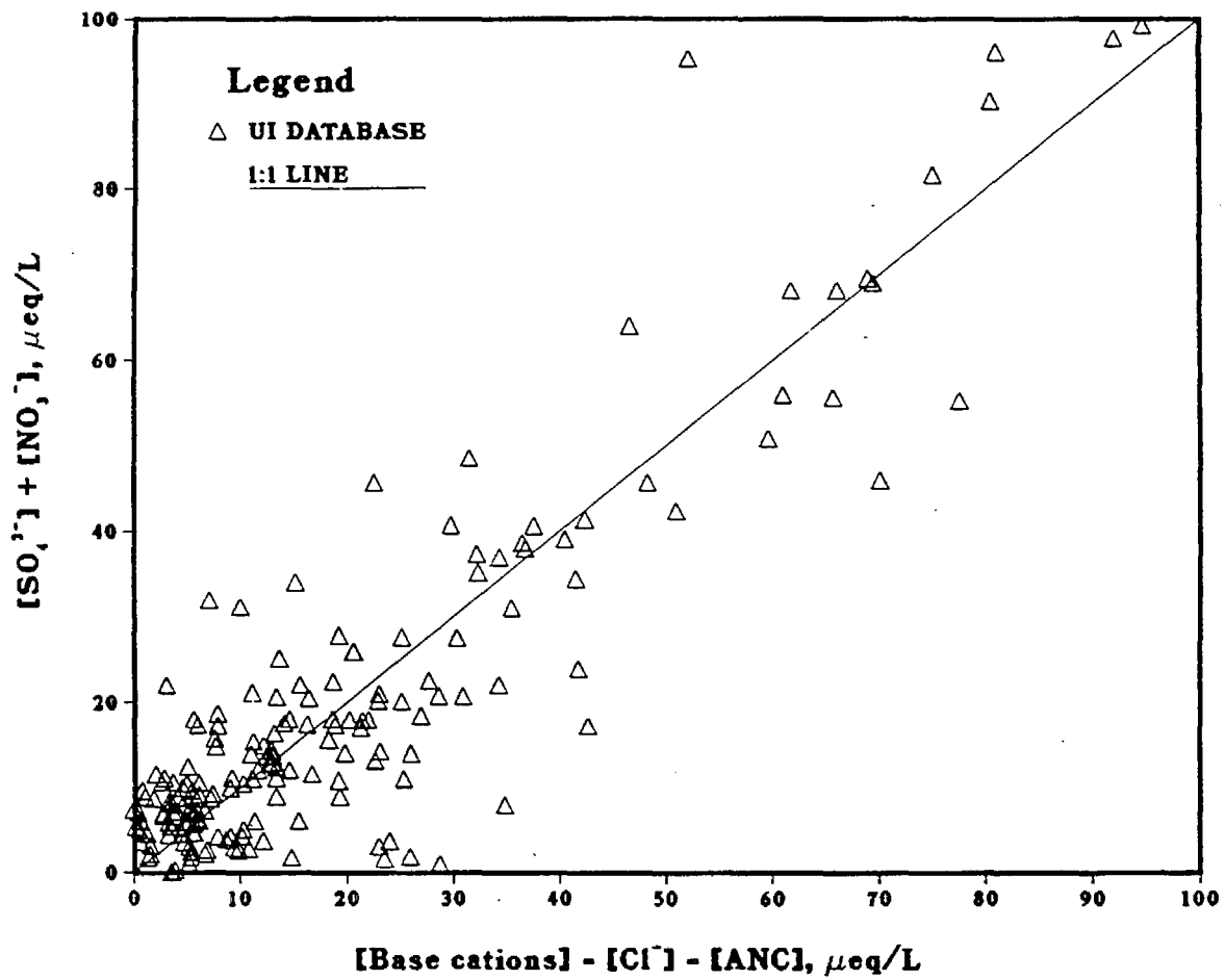
Figure 11. Lake sulfate and nitrate versus the sum of the base cations (corrected for ocean sources of sodium) minus ANC.
