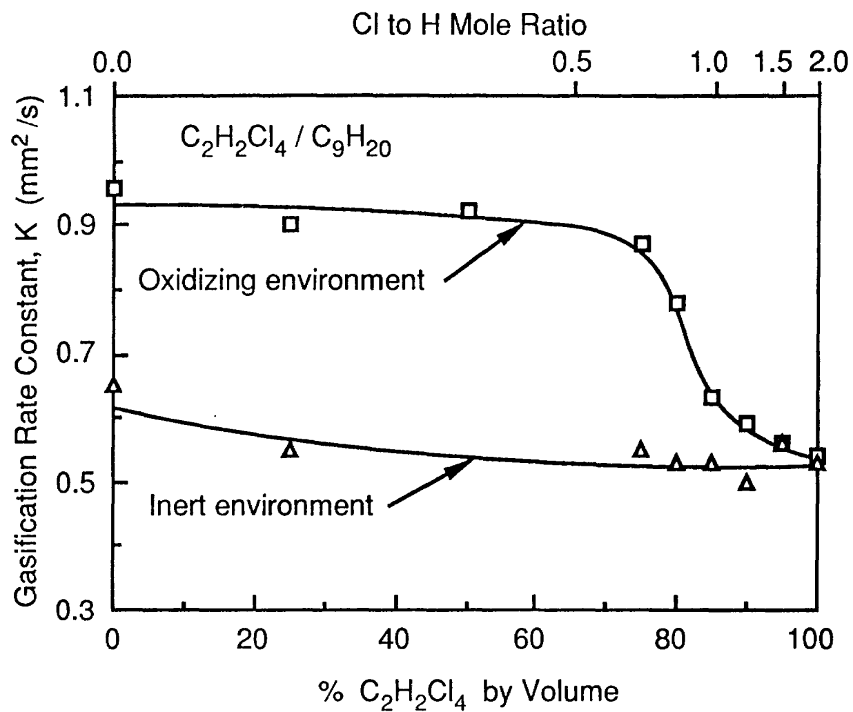
Figure 9. Gasification rate constants of tetrachloroethane/nonane droplet mixtures in oxidizing and inert environments.
