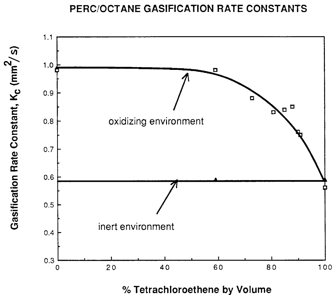
Figure 15. Gasification rate constants of tetrachloroethene/octane droplet mixtures in oxidizing and inert environments.
