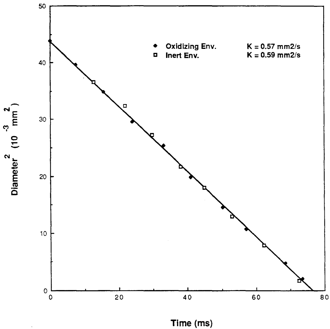
Figure 14. Gasification profile of tetrachloroethene droplets injected into oxidizing and inert environments.
