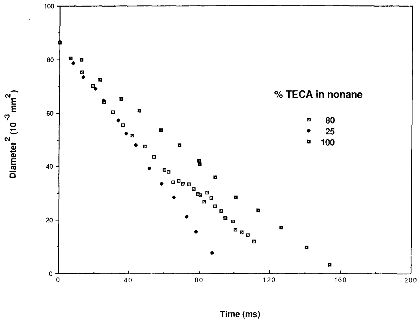
Figure 8. Gasification profiles of droplets of 25%, 80%, 100% tetrachloroethane (by volume) in nonane injected into an oxidizing environment.
