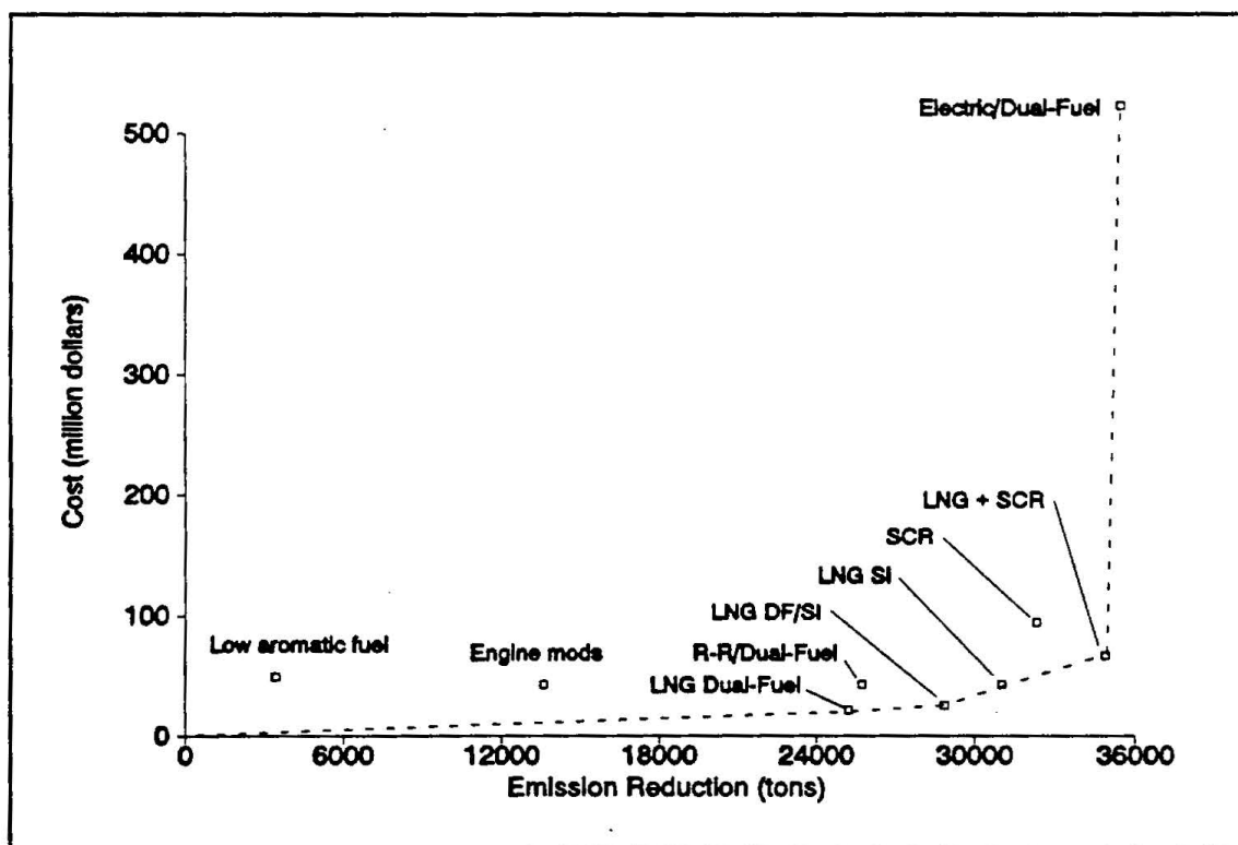
Figure 3: Cost vs. emission reduction for potential line-haul, local, and switcher locomotive control measures.
