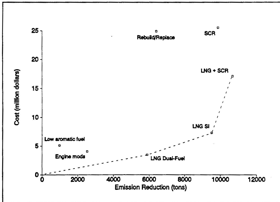
Figure 2: Cost vs. emission reduction for potential local and yard locomotive control measures.
