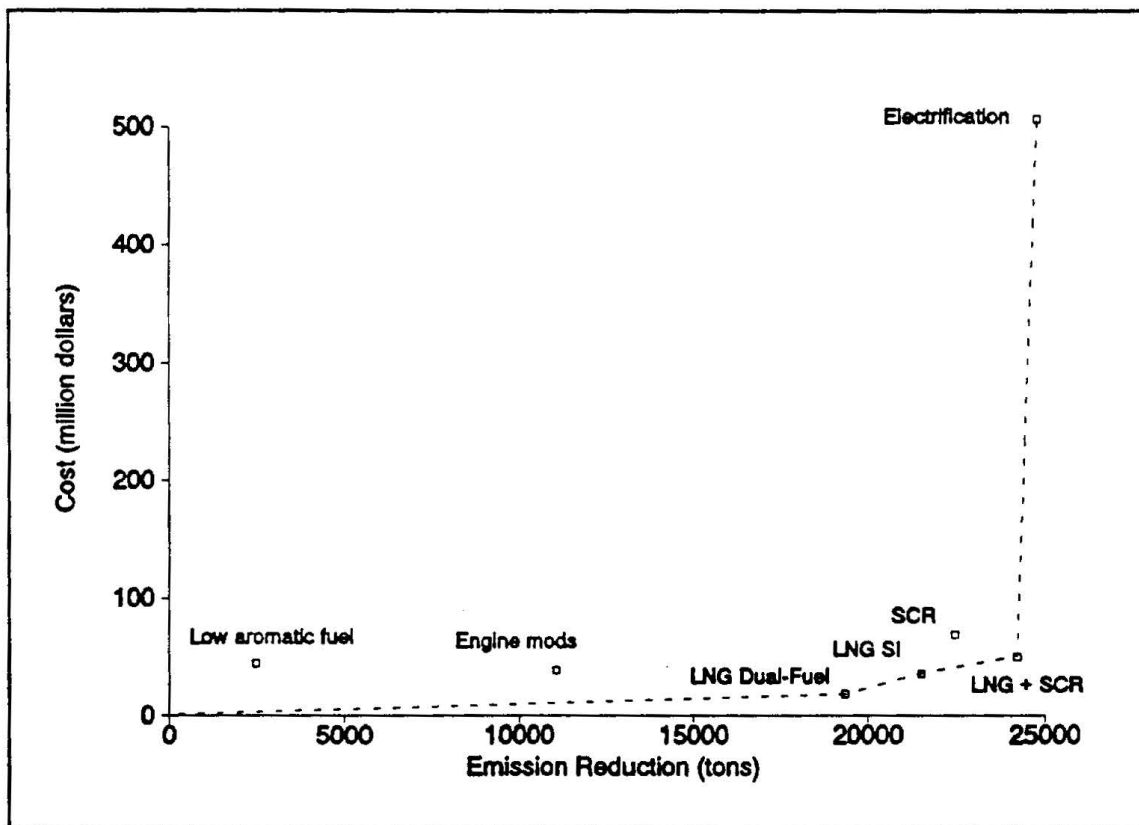
Figure 1: Cost vs. emission reduction for potential line-haul locomotive control measures.
