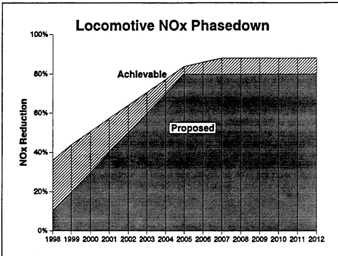
Figure 4: Proposed locomotive NOx phasedown schedule vs. technologically achievable reduction.
