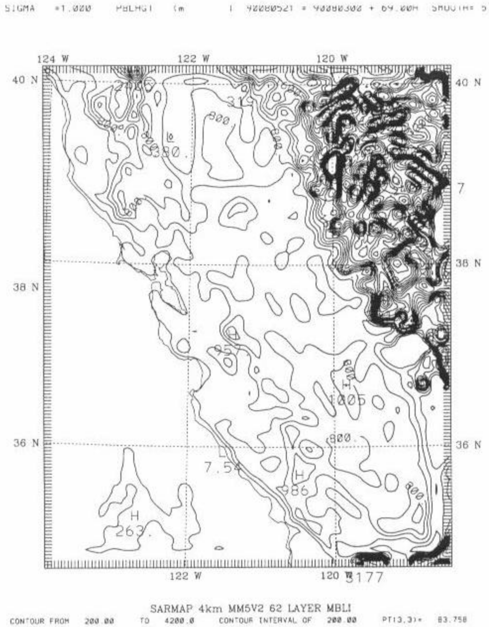
Figure 29. Mixed-layer depth (m) simulated by the MM5 at 0000 UTC 6 August 1990 in the 4-km domain for Exp. 1. Contour interval is 200 m.
