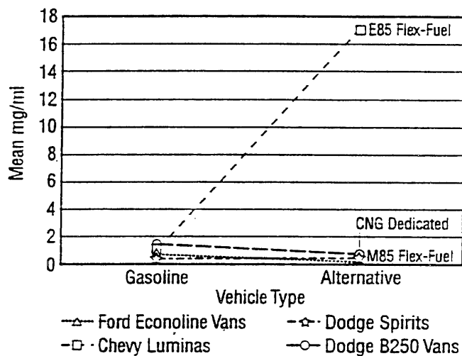
Figure 7. Comparison of CH 3 CHO emissions from four light-duty AFVs and their gasoline-fueled counterparts.
