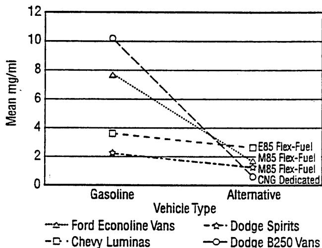
Figure 4. Comparison of C_6H_6 emissions from four light-duty AFVs and their gasoline-fueled counterparts.
