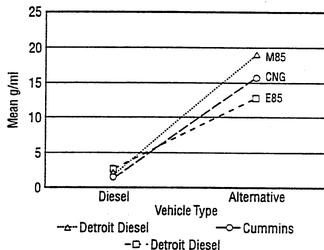
Figure 11. Comparison of HC emissions from three alternative fuel transit buses and their diesel-fueled counterparts.
