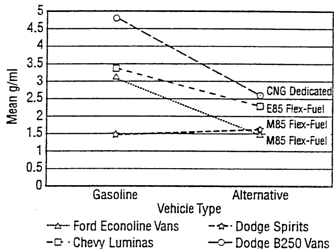
Figure 1. Comparison of CO emissions from four light-duty AFVs and their gasoline-fueled counterparts.
