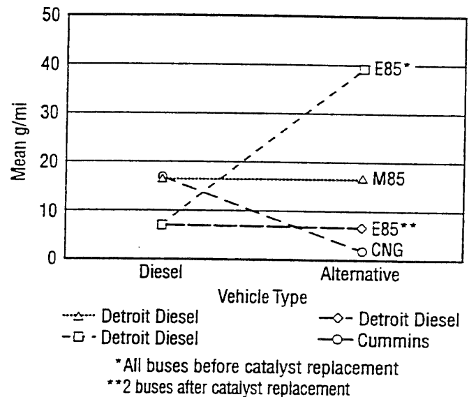
Figure 9. Comparison of CO emissions from three alternative fuel transit buses and their diesel-fueled counterparts.
