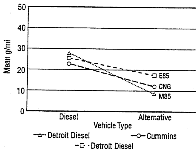
Figure 10. Comparison of \text{NO}_x emissions from three alternative fuel transit buses and their diesel-fueled counterparts.
