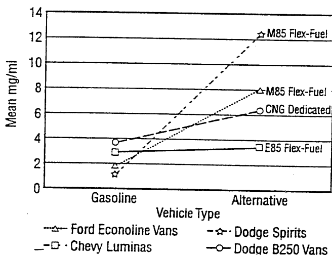
Figure 6. Comparison of HCHO emissions from four light-duty AFVs and their gasoline-fueled counterparts.
