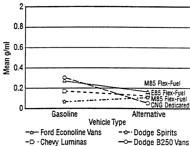
Figure 3. Comparison of HC emissions from four light-duty AFVs and their gasoline-fueled counterparts.
