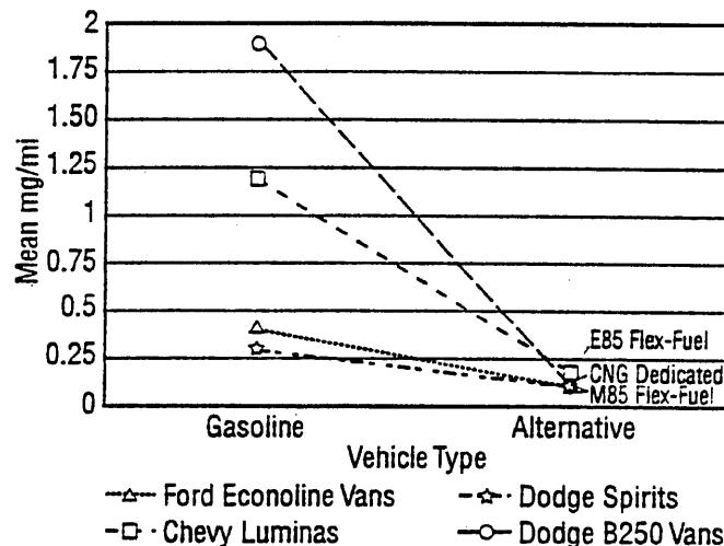
Figure 5. Comparison of C_4H_6 emissions from four light-duty AFVs and their gasoline-fueled counterparts.
