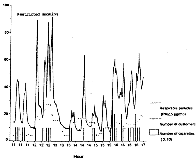
Figure 1. Estimated PM 2.5 concentrations (from light scattering measurements), customer and cigarette counts inside restaurant with restricted smoking.
