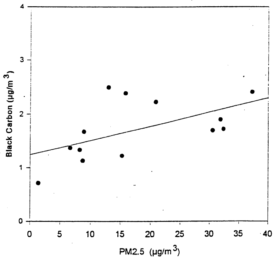
Figure 3. Black Carbon vs. PM2.5 (Regression line is shown).
