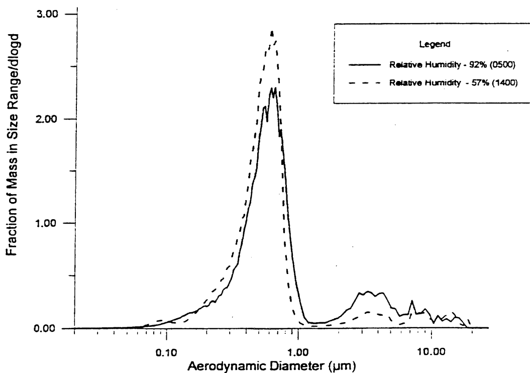
Figure 5. Typical Distribution of Particle Mass, 0.02 to 10 m. Aerodynamic Diameter
