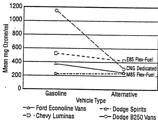
Figure 8. Comparison of OFP from four light-duty AFVs and their gasoline-fueled counterparts.
