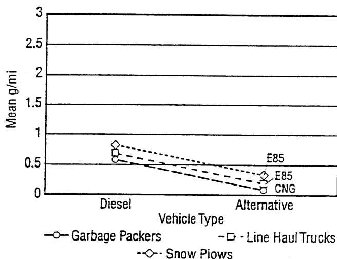
Figure 13. Comparison of PM emissions from three heavy-duty AFVs and their diesel-fueled counterparts.
