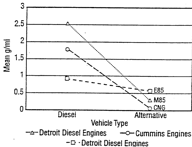
Figure 12. Comparison of PM emissions from three alternative fuel transit buses and their diesel-fueled counterparts.
