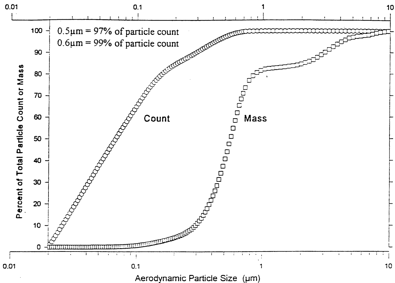
Figure 4. Typical Distribution of Cumulative Particle Counts and Mass, 0.02 to 10 m.
