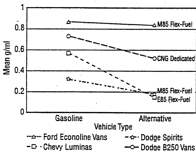
Figure 2. Comparison of \text{NO}_x emissions from four light-duty AFVs and their gasoline-fueled counterparts.
