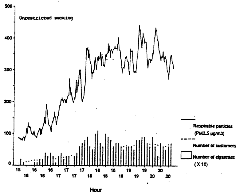
Figure 3. Estimated PM 2.5 concentrations (from light scattering measurements), customer and cigarette counts inside unrestricted smoking restaurant / bar.
