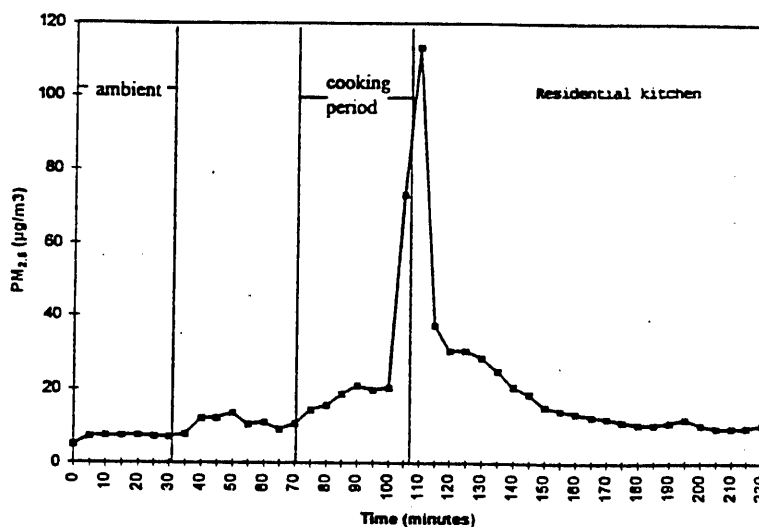
Figure 4. Estimated PM 2.5 concentration inside a residential kitchen with a 34 minute cooking period.
