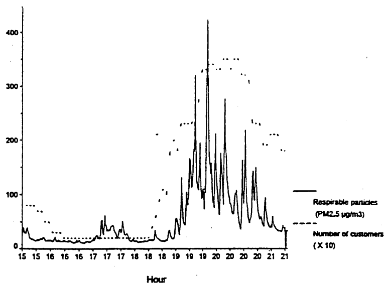
Figure 2. Estimated PM 2.5 concentrations (from light scattering measurements) and customer counts inside non-smoking restaurant.
