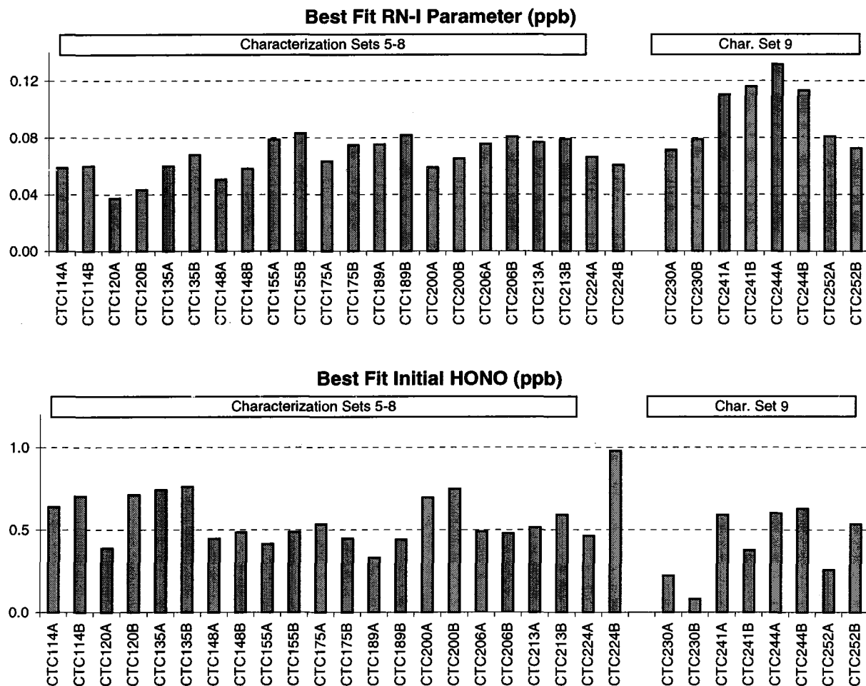
Figure 9. Radical source parameters that gave the best fits to the results of the n-butane - NO x and CO - NO x experiments used to characterize the conditions of the CTC during the period of this project.
