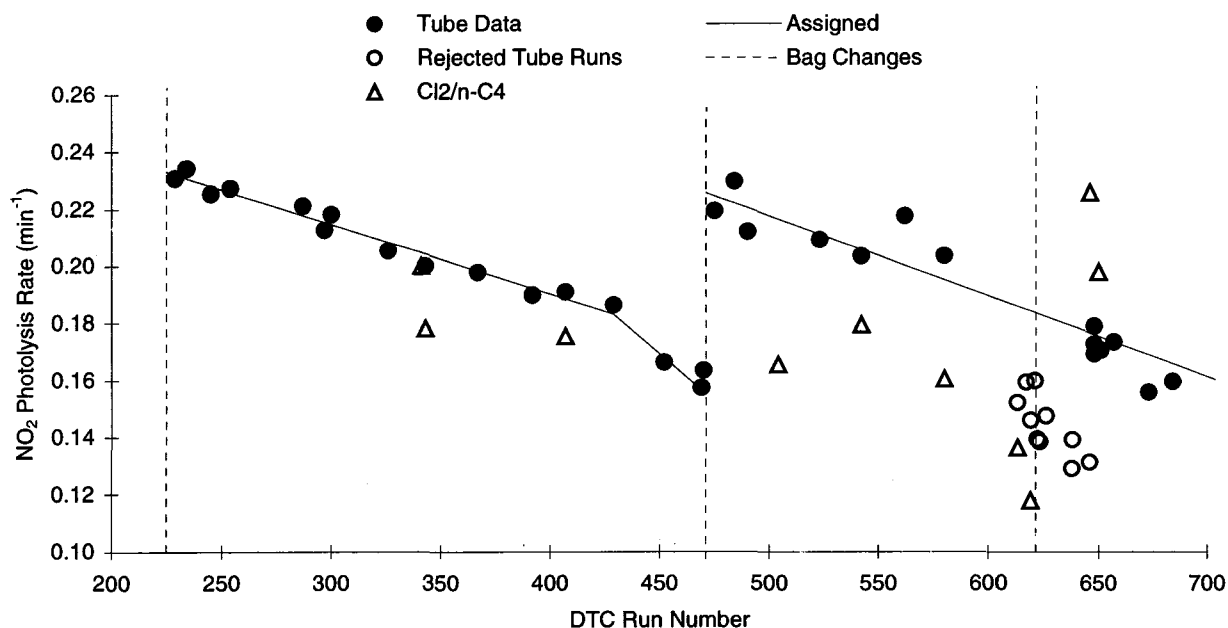
Figure 5. Plots of results of actinometry experiments against DTC run number, showing \text{NO}_2 photolysis rate assignments used for modeling purposes.
