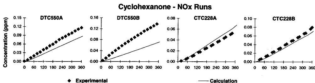
Figure 17. Plots of experimental and calculated \Delta([O_3]-[NO]) results for the cyclohexanone - NO x experiments.
