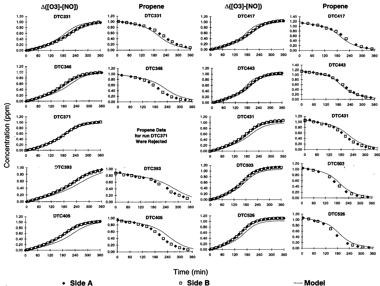
Figure 10. Experimental and calculated concentration-time plots for the \Delta([O_3]-[NO]) and propene data in the propene - NO_x control experiments in the DTC.
