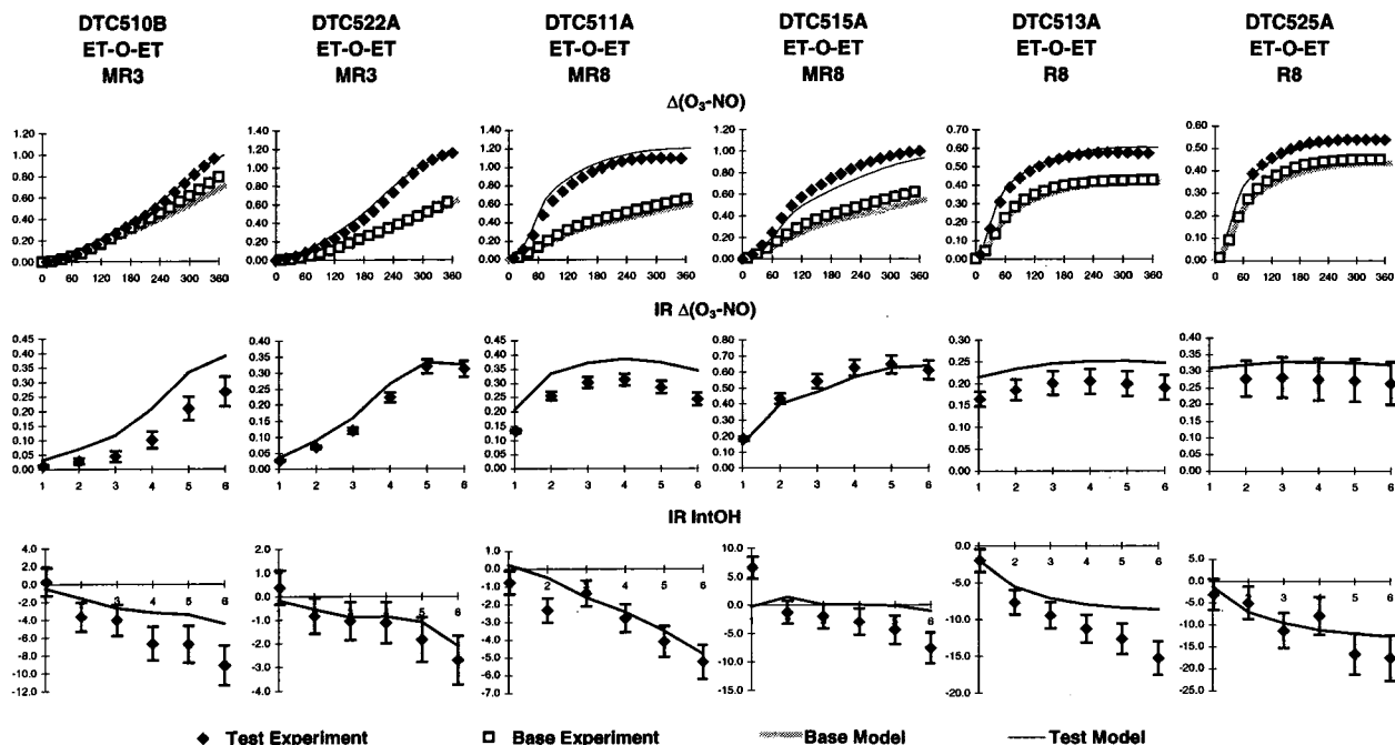
Figure 23. Plots of experimental and calculated results of the incremental reactivity experiments with diethyl ether.
