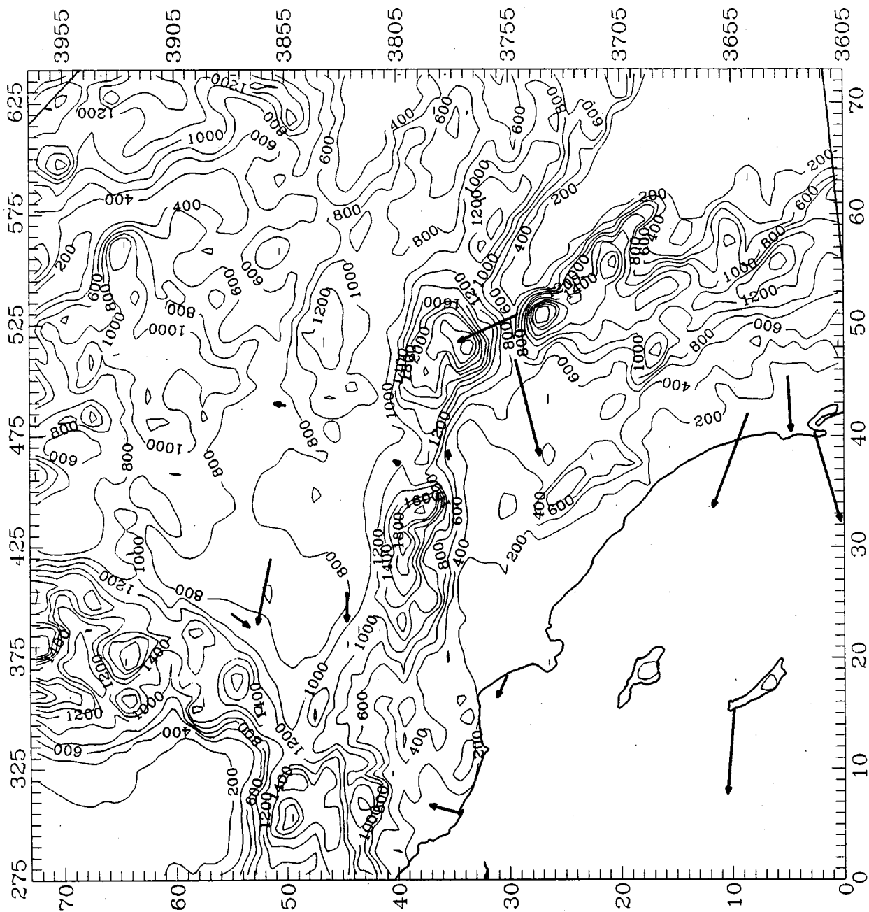
Averaged Wind Observations For Days Classified As M-L
