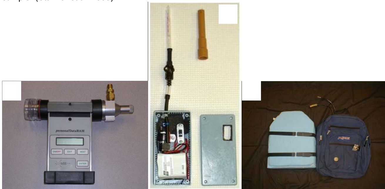
Figure 1. Personal exposure monitor. A. Personal DataRAM model 1200 with PM_{2.5} cyclone inlet and filter cassette at outlet (MIE Inc., Bedford, MA). B. Personal NO_2 monitor with a miniaturized diaphragm pump and triethanolamine-treated molecular sieve sorbent tubes (SKC, Fullerton, CA). C. Backpack for the PEM with sound-insulated foam encasement.
