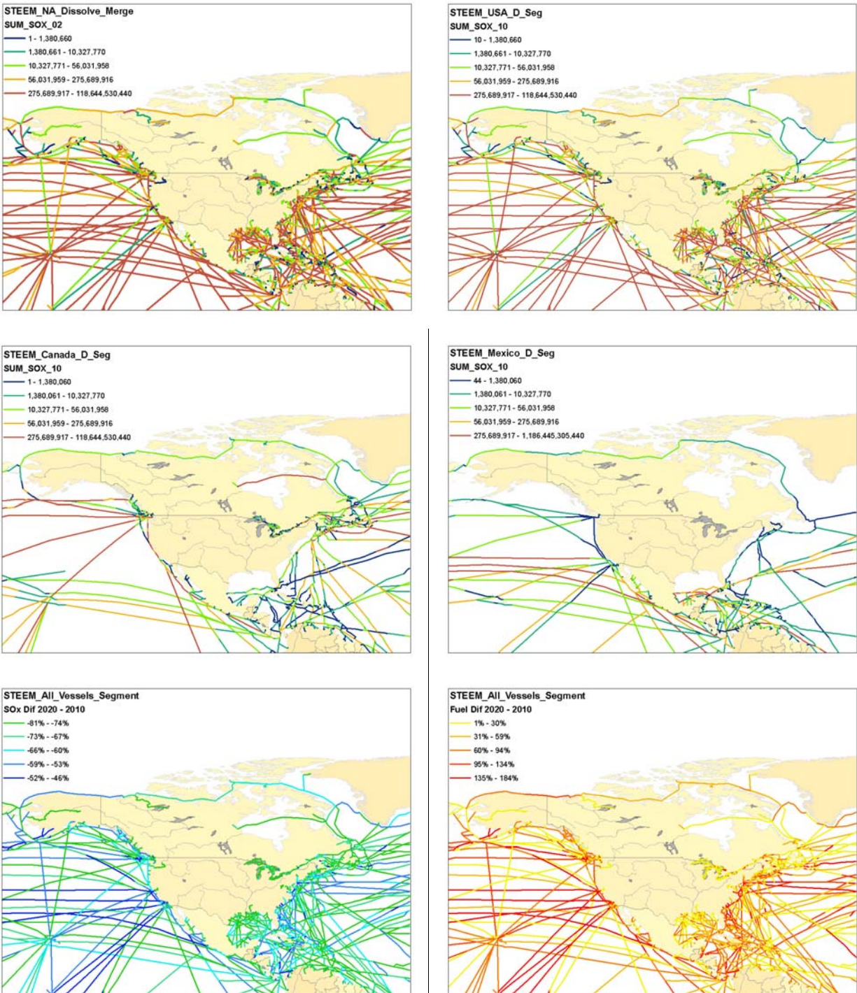
Figure 4. STEEM results for a) 2002 data provided for all ships; and 2010 results under Scenario 1 for b) US data; c) Canada data; and d) Mexico data; and comparison of 2020 and 2010 for e) SO x and f) Fuel use.
