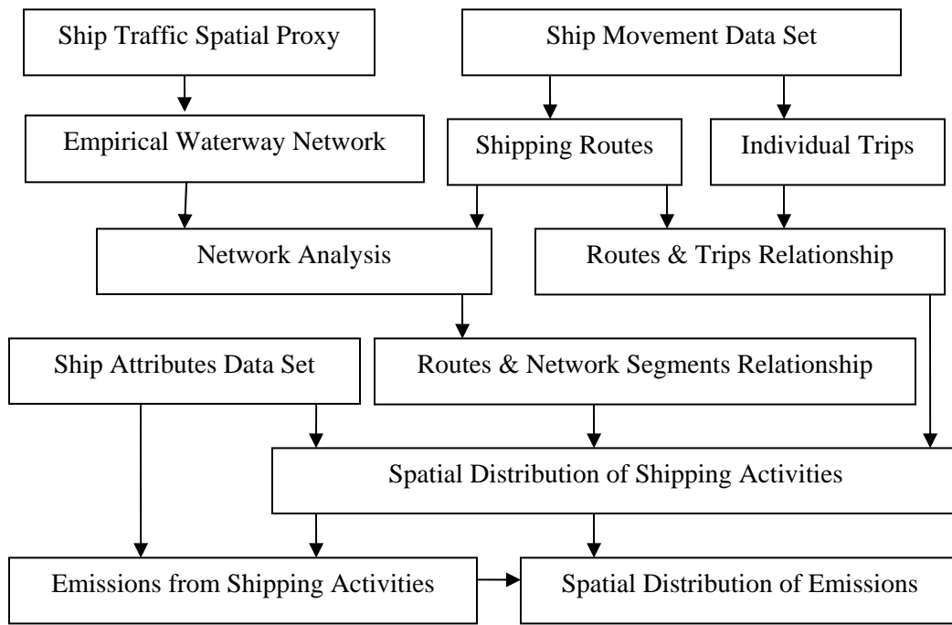
Figure 1. Illustration of Waterway Network Ship Traffic, Energy and Environment Model (STEEM) as applied to emission estimation.
