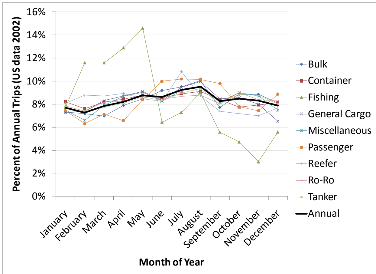
Figure 6. Monthly variation in emissions from North American Ship Traffic
