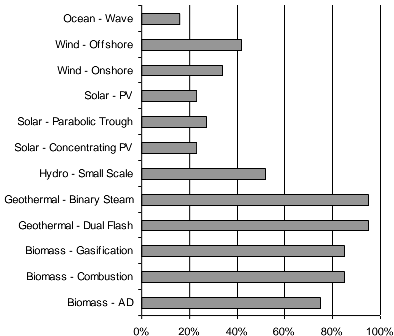
Figure 130 Capacity Factors for Selected Renewables (Average Net Capacity %)
