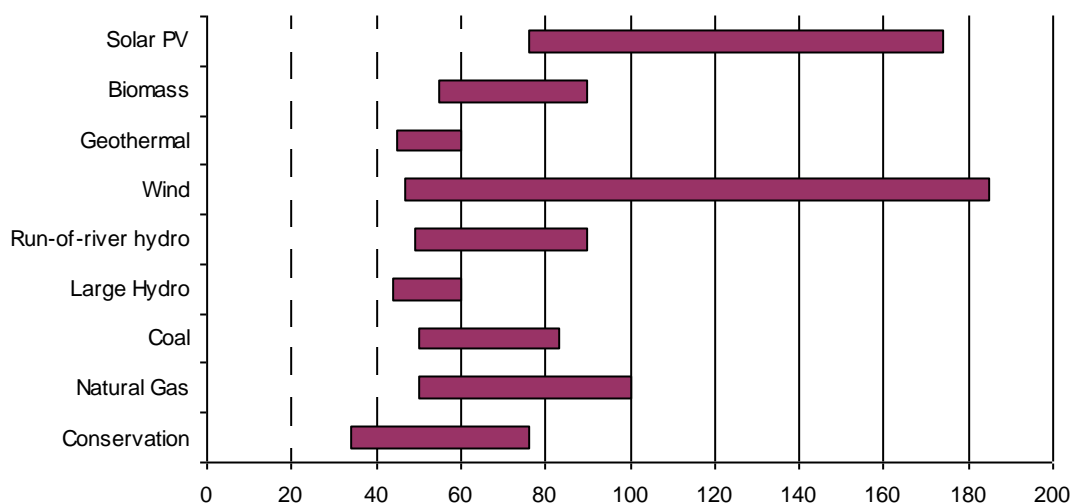
Figure 131 Levelized Costs: Generation Cost Range ($/MWh)
