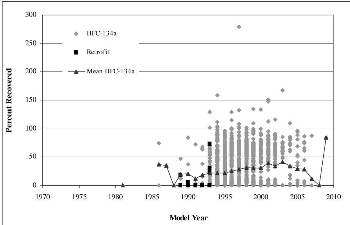
Figure 36: Recovered Refrigerant of 1,842 Round Two Vehicles
