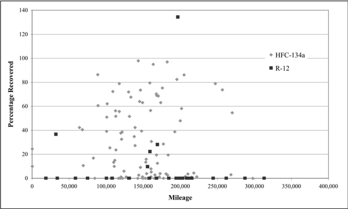
Figure 27: Recovered Refrigerant and Mileage of Initial 160 Sampled Vehicles
