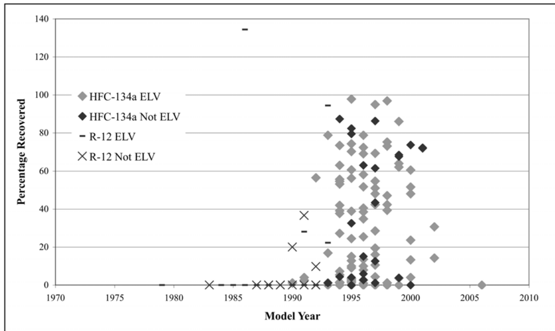
Figure 28: Recovered Refrigerant by Model Year and CA DMV Status of Initial 160 Sampled Vehicles
