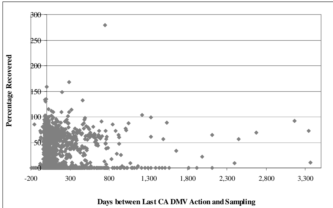
Figure 43: Percentage HFC-134a Recovered and Time Elapsed Between Last CA DMV Status and Sampling for 1,842 Round Two Vehicles
