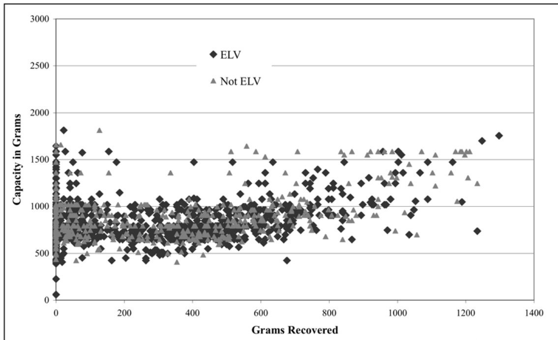
Figure 45: HFC-134a Capacity and HFC-134a Recovered in Grams for 1,842 Round Two Vehicles
