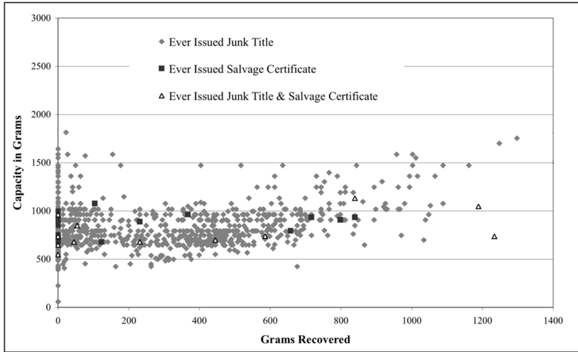
Figure 46: HFC-134a Capacity and HFC-134a Recovered for 1,242 Round Two ELVs
