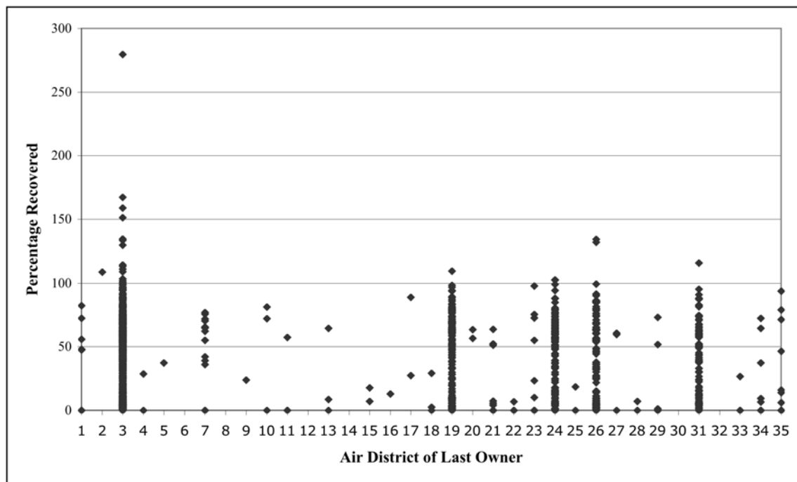
Figure 55: Percentage Refrigerant Recovered by Air District of Last Known Owner for 1,802 Samples with CA DMV Registration Status
