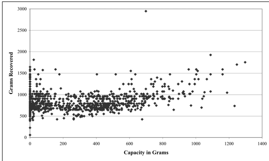
Figure 65: HFC-134a Capacity and Grams Recovered for 1,340 Sampled ELVs
