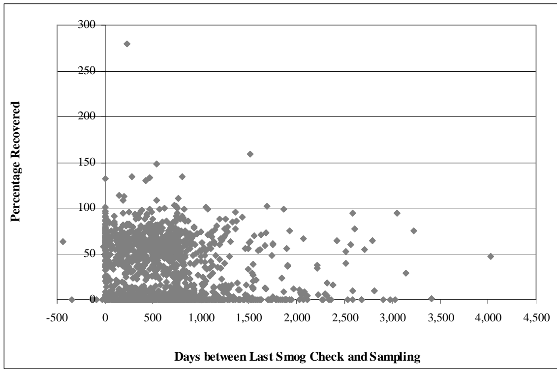
Figure 57: Percentage Recovered and Days Between Last Smog Check and Sampling for 1,695 Sampled Vehicles with a Smog Check Record
