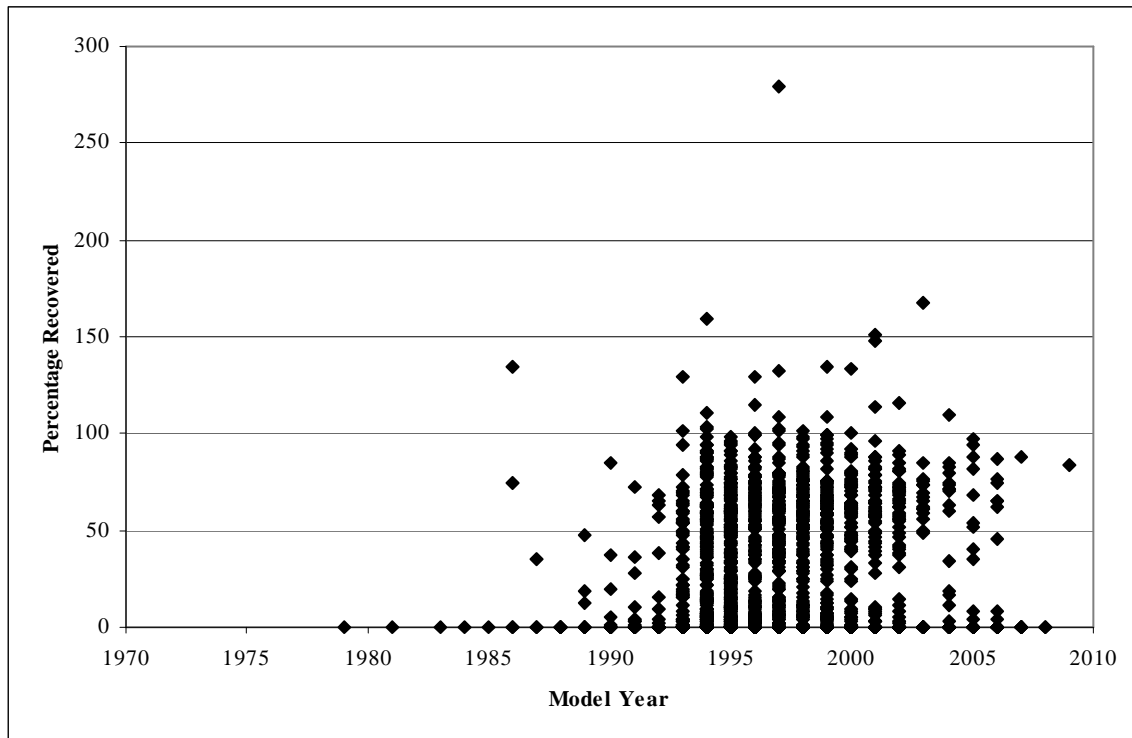
Figure 49: Recovered Refrigerant for 2,002 Sampled Vehicles
