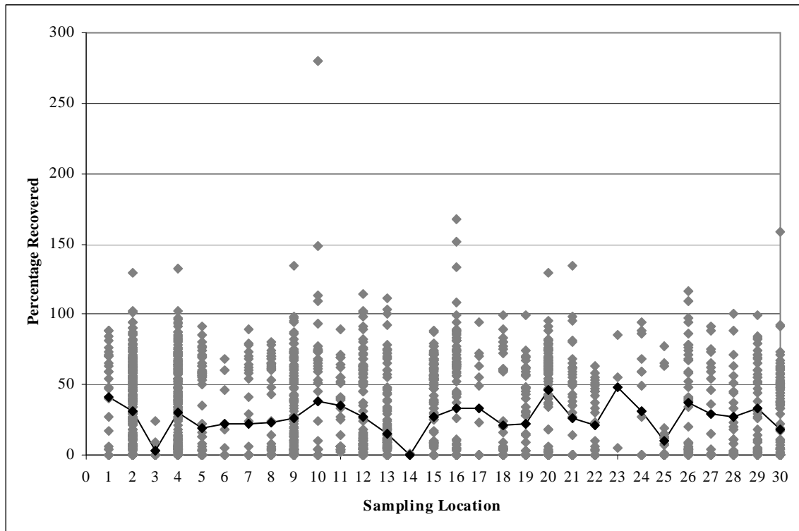
Figure 53: Percentage Recovered by Sampling Location for 2,002 Sampled Vehicles
