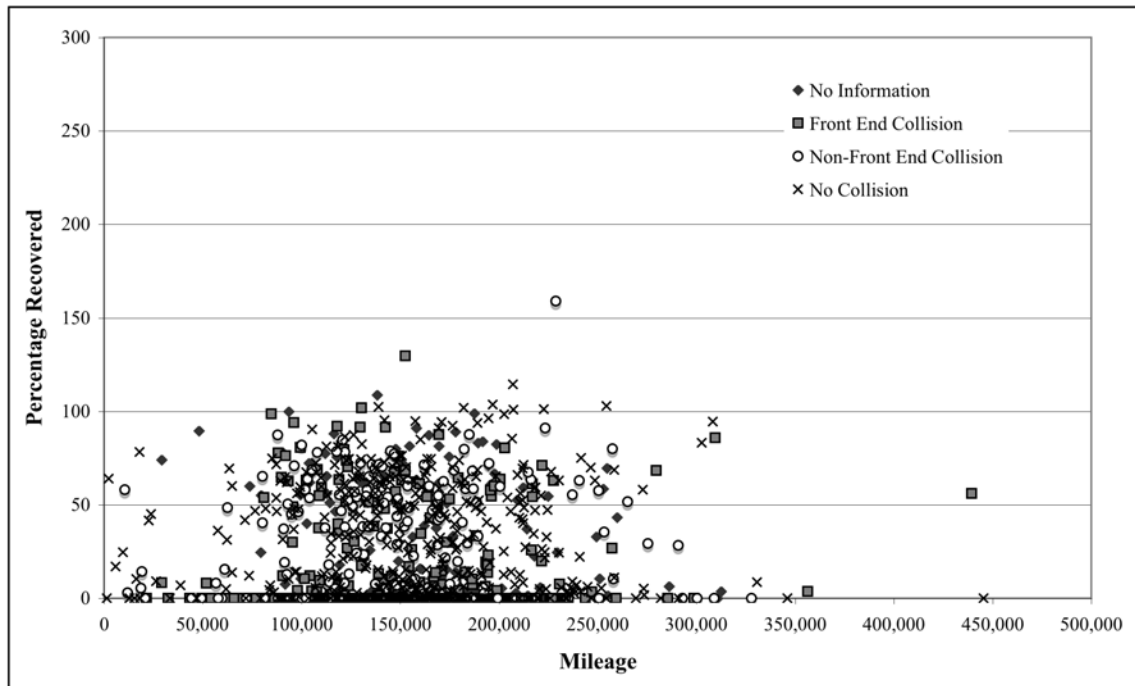
Figure 37: Recovered Refrigerant and Mileage for 1,842 Round Two Vehicles
