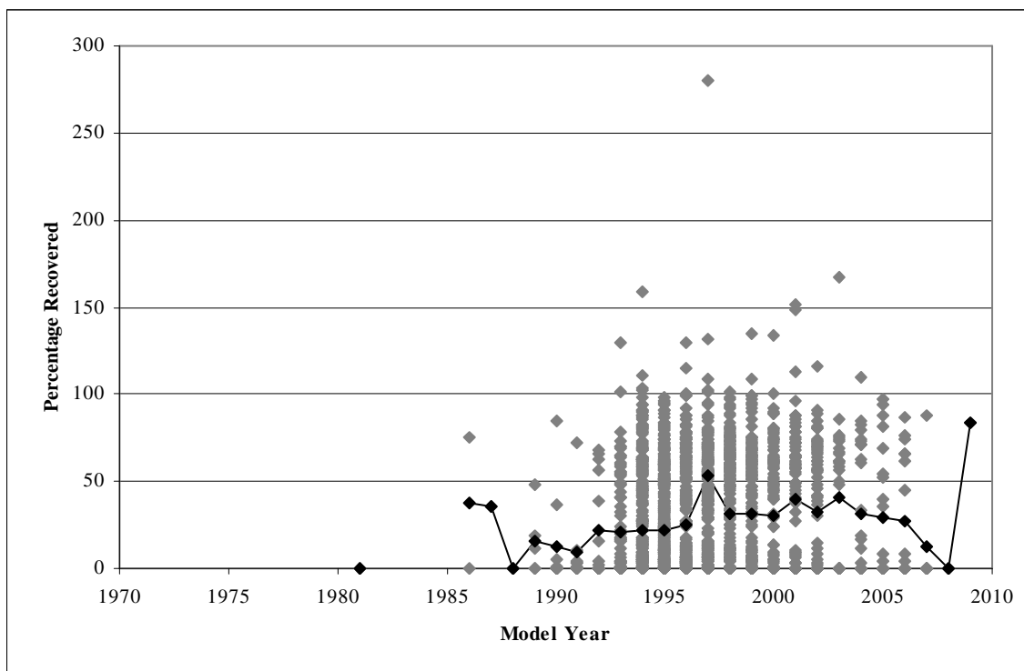
Figure 63: Percentage of HFC-134a Recovered from 1,966 Sampled Vehicles
