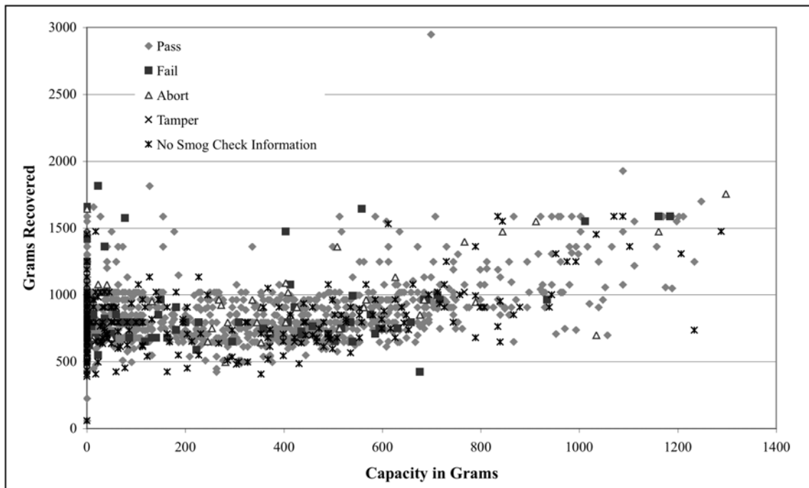
Figure 56: Recovered and Capacity Refrigerant by Last Smog Check Result for 2,002 Sampled Vehicles
