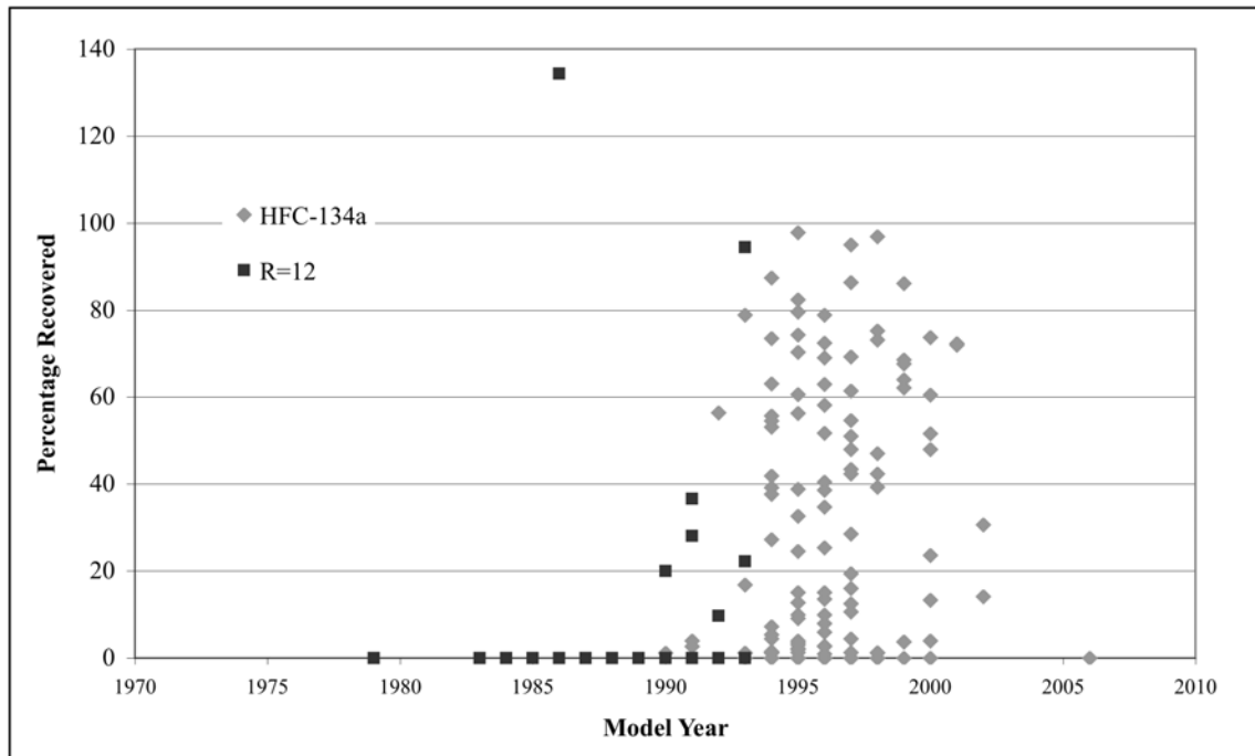
Figure 23: Percentage of Refrigerant Remaining in Initial 160 Sampled Vehicles
