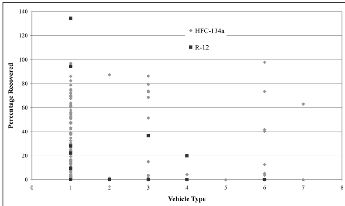
Figure 26: Percentage Refrigerant Recovered by Vehicle Type of Initial 160 Sampled Vehicles
