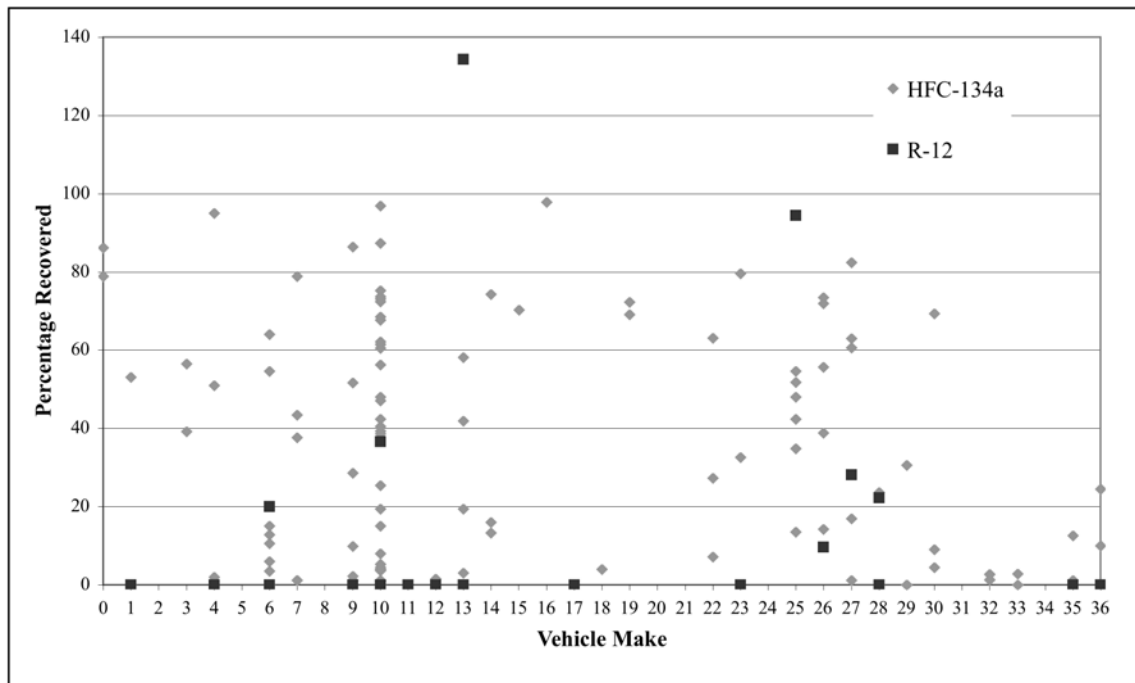
Figure 24: Percentage Refrigerant Recovered by Vehicle Make of Initial 160 Sampled Vehicles
