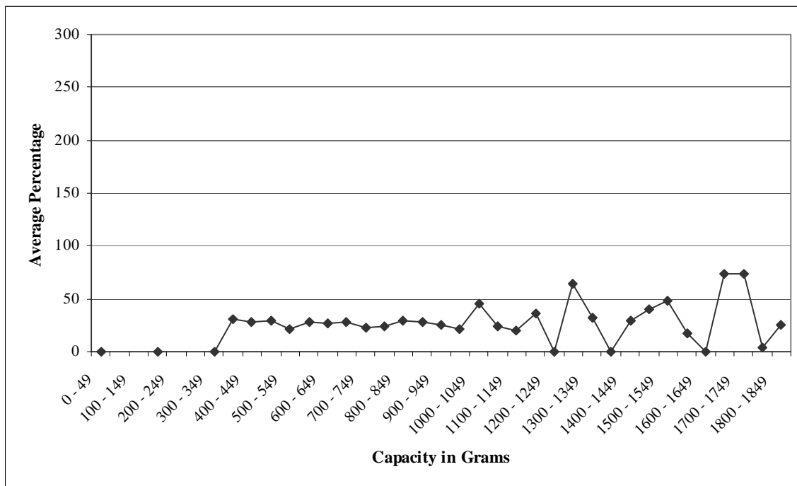
Figure 47: Average Recovered Refrigerant Across Capacity Partitions for 1,842 Round Two Vehicles
