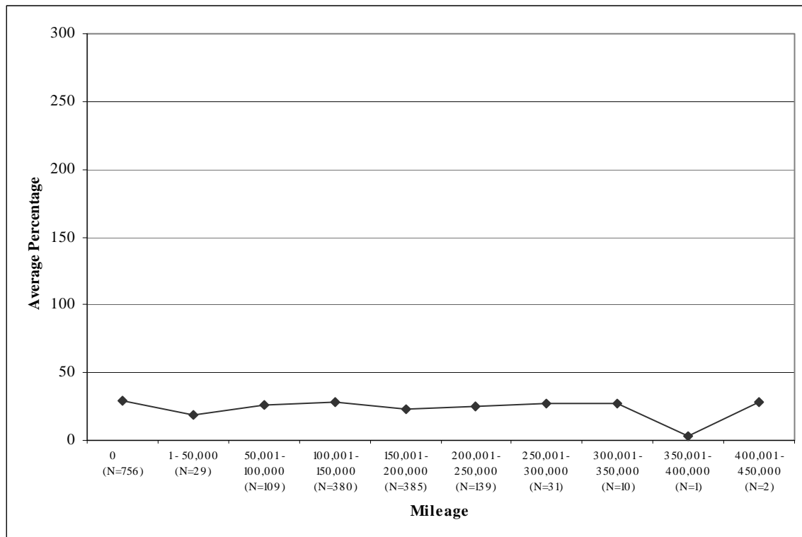
Figure 38: Average Recovered Refrigerant Across Mileage Partitions for 1,842 Round Two Vehicles
