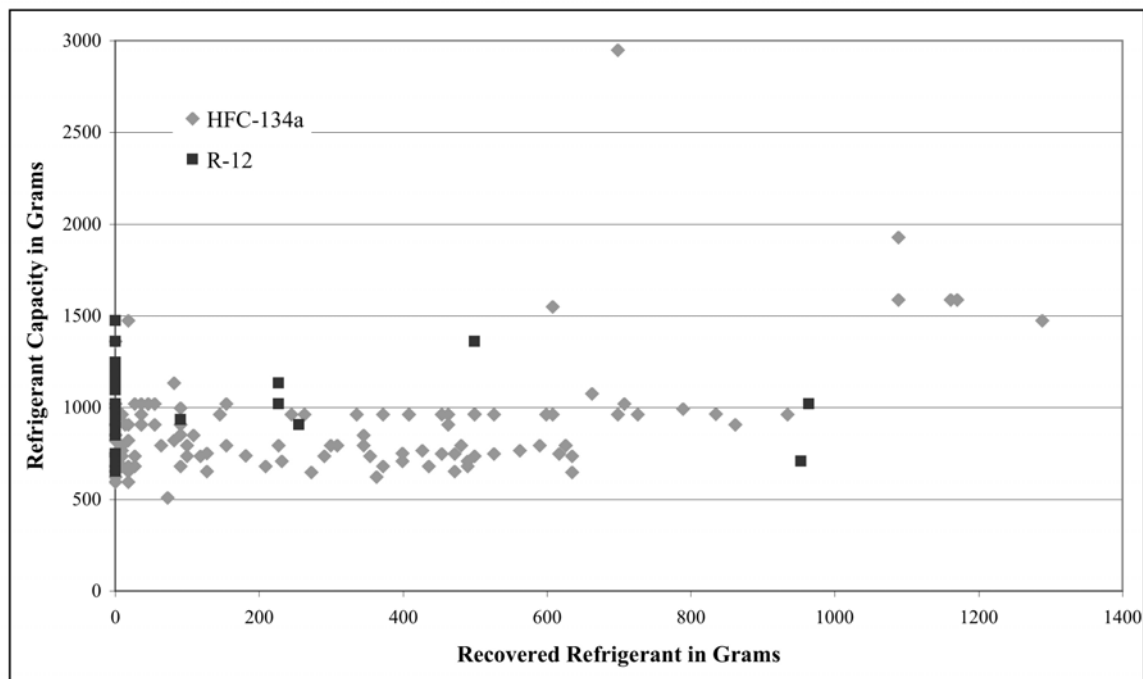
Figure 30: Refrigerant Capacity and Recovered Refrigerant of Initial 160 Sampled Vehicles
