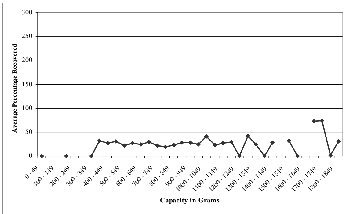
Figure 66: Average Recovered HFC-134a Across Capacity Partitions for 1,340 Sampled ELVs
