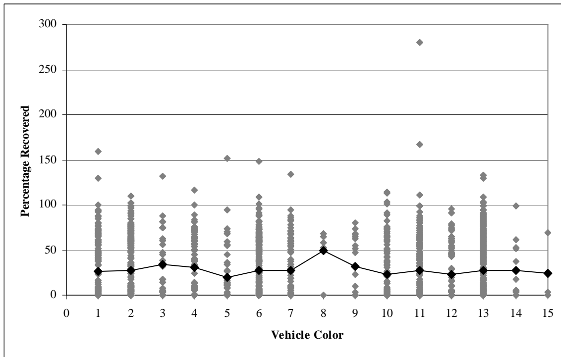
Figure 40: Percentage of Recovered HFC-134a and Vehicle Color for 1,842 Round Two Vehicles
