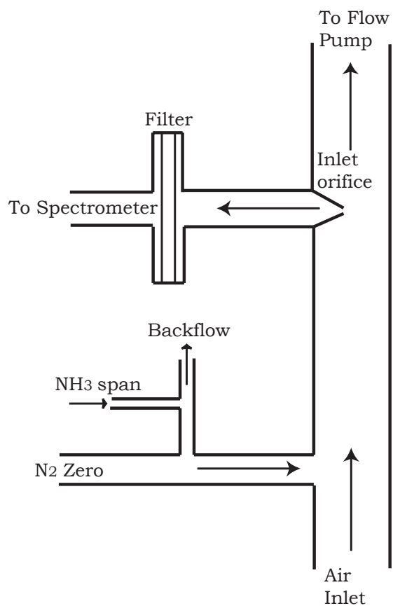
Fig 2. Schematic illustration of the air sampling manifold with critical orifice flow inlet and air filter. Automated instrument zero and span calibrations are performed by periodically flowing N_2 into inlet, either without or with the addition of NH_3 from a permeation tube source.
