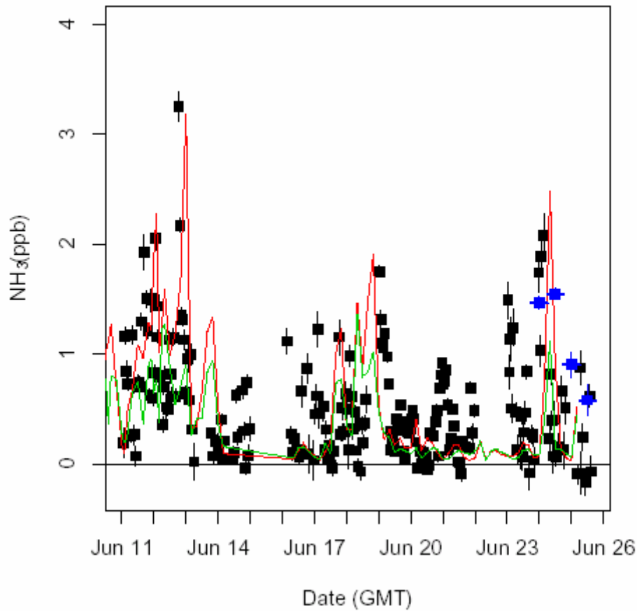
Figure 11. Measured hourly \text{NH}_3 mixing ratios from LBNL system (black points), DRI 12 hour integrated sampler results (blue points), and predicted \text{NH}_3 mixing ratios predicted from the back trajectory calculations and cattle-only \text{NH}_3 emission inventory. Predicted \text{NH}_3 is scaled to fit on plot so that \text{NH}_3 predicted without deposition (red line) is scaled by a factor of 0.5, while \text{NH}_3 predicted with deposition (green line) is scaled by a factor of 2.
