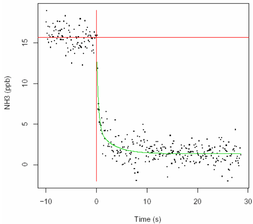
Fig 3. Time series of \text{NH}_3 mixing ratio showing transient decay following removal of \text{NH}_3 span gas from zero air flow to instrument inlet.
