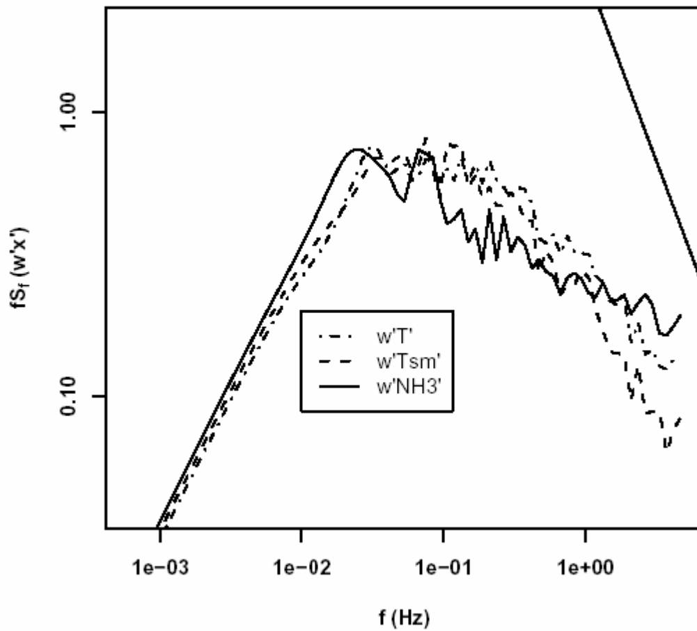
Figure 7. Power spectra of covariance in vertical wind speed with sonic temperature, w'T' , smoothed sonic temperature, w'T'_{sm} , and fluctuations in NH_3 mixing ratio, w'NH_3' . The straight line in upper right shows -4/3 slope expected for fluctuation spectra in an inertial sublayer.
