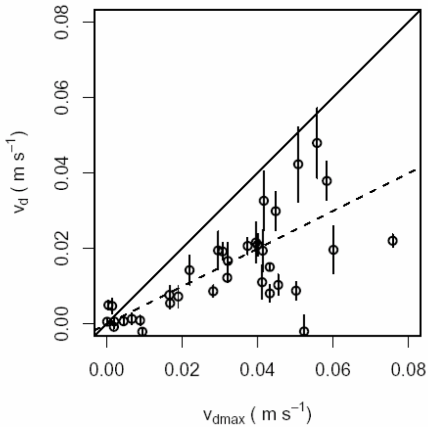
Figure 9. Scatter plot comparison of measured deposition velocity, v_d , and maximum deposition velocity in the case that all molecules reaching the leaf surface are absorbed, v_{dmax} .
