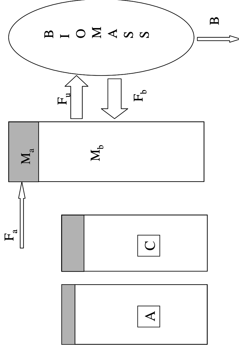
Figure 11. A box model representation of nitrate cycling in Lake Tahoe. New inputs of nitrate are from atmospheric deposition ( F_a ) and losses of N are through organic burial (B). Internal recycling of nitrate via uptake ( F_u ) and nitrification ( F_b ) control the balance of nitrate in the water column. Water column nitrate \Delta^{17}\text{O} values reflect the relative rate of F_a and F_b . Should the deposition rate decrease because of regulatory efforts, what would the effect on the cycle be? The response budgets for lake nitrate sources are shown in A and C. The initial response is isotopic disequilibrium relative to the initial conditions. This is shown in A, where the \Delta^{17}\text{O} values has shrunk along with the deposition loading decrease (box size, not to scale). This is expected because F_u and F_b depend on the amount of the water column algae (Biomass) and therefore one expects F_b not to be immediately impacted by a small change in F_a . A small shift in deposition only results in a small shift total nitrate, biomass remains effectively unchanged on short timescales, and thus F_b remains unchanged. Over time both biomass and F_b , and F_u will adjust, assuming constant burial. If the shrinkage of biomass is proportional to the deposition decrease, the system should equilibrate isotopically but with a different nitrate concentration (box C). If the system is not directly proportional to deposition, the isotopic balance would end up somewhere between A and C. Long term monitoring of water column nitrate \Delta^{17}\text{O} is thus an effective proxy for changes in lake algal biomass and could trace spatial productivity inhomogeneities across the lake.
