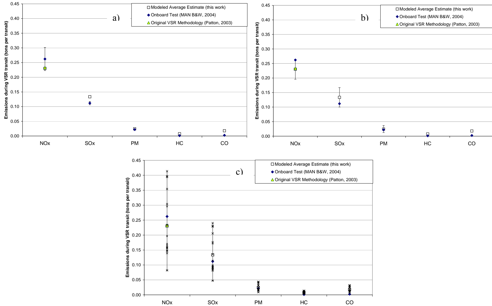
Figure 3. Comparison of transit emissions estimates with modeled and measured average emissions factors a) Applying measurement uncertainty reported for emission factors [MAN B&W Diesel A/S, 2004]; b) Applying uncertainty estimates from emission factor summaries [Cooper, 2004]; and c) Demonstrating variability among transit estimates at different speeds. All transit estimates represent the Sine Maersk.
