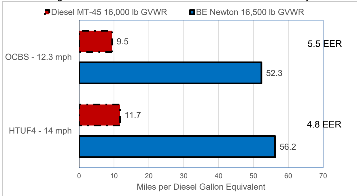
Figure 4: CalHEAT Parcel Van Diesel vs Electric Fuel Efficiency
