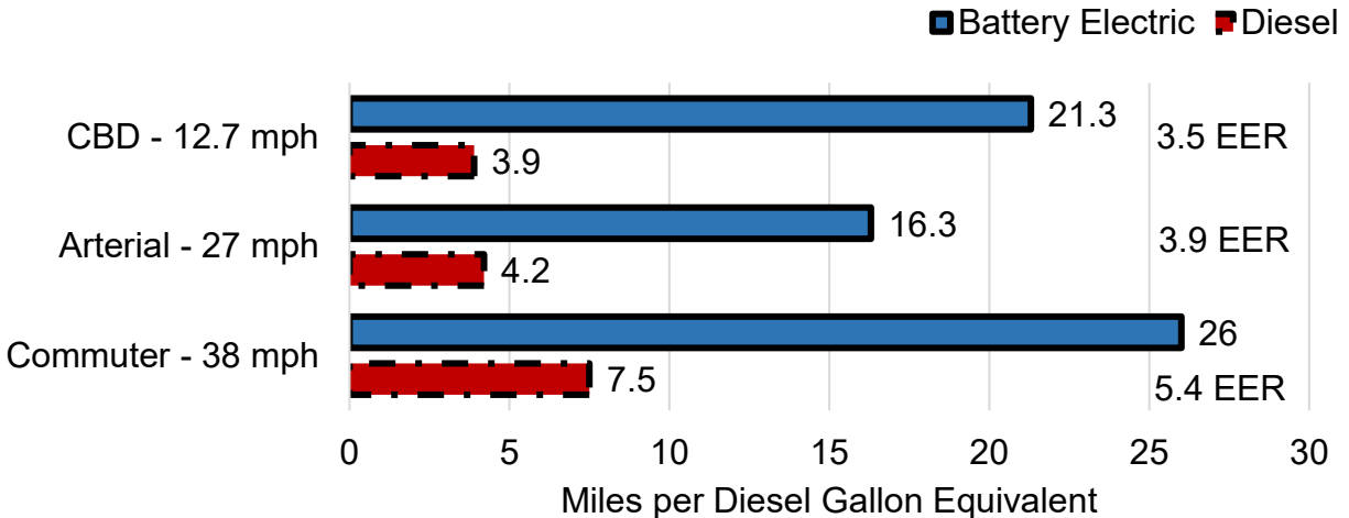
Figure 2: Altoona Buses Diesel vs Electric Fuel Efficiency (Test Cycle)
