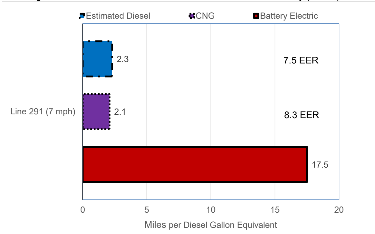
Figure 6: Foothill Transit Bus Fleet CNG vs Electric Fuel Efficiency (In-Use)
