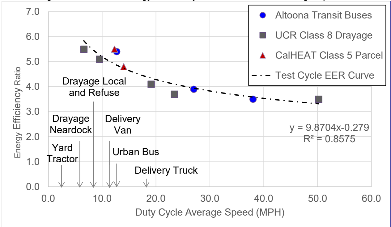
Figure 11: Vehicle Energy Efficiency Ratio at Different Average Speeds
