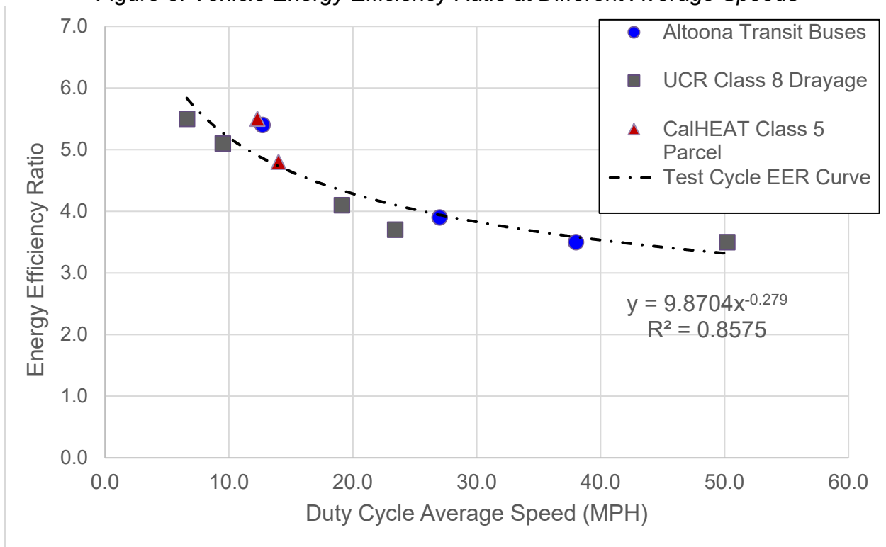
Figure 5: Vehicle Energy Efficiency Ratio at Different Average Speeds
