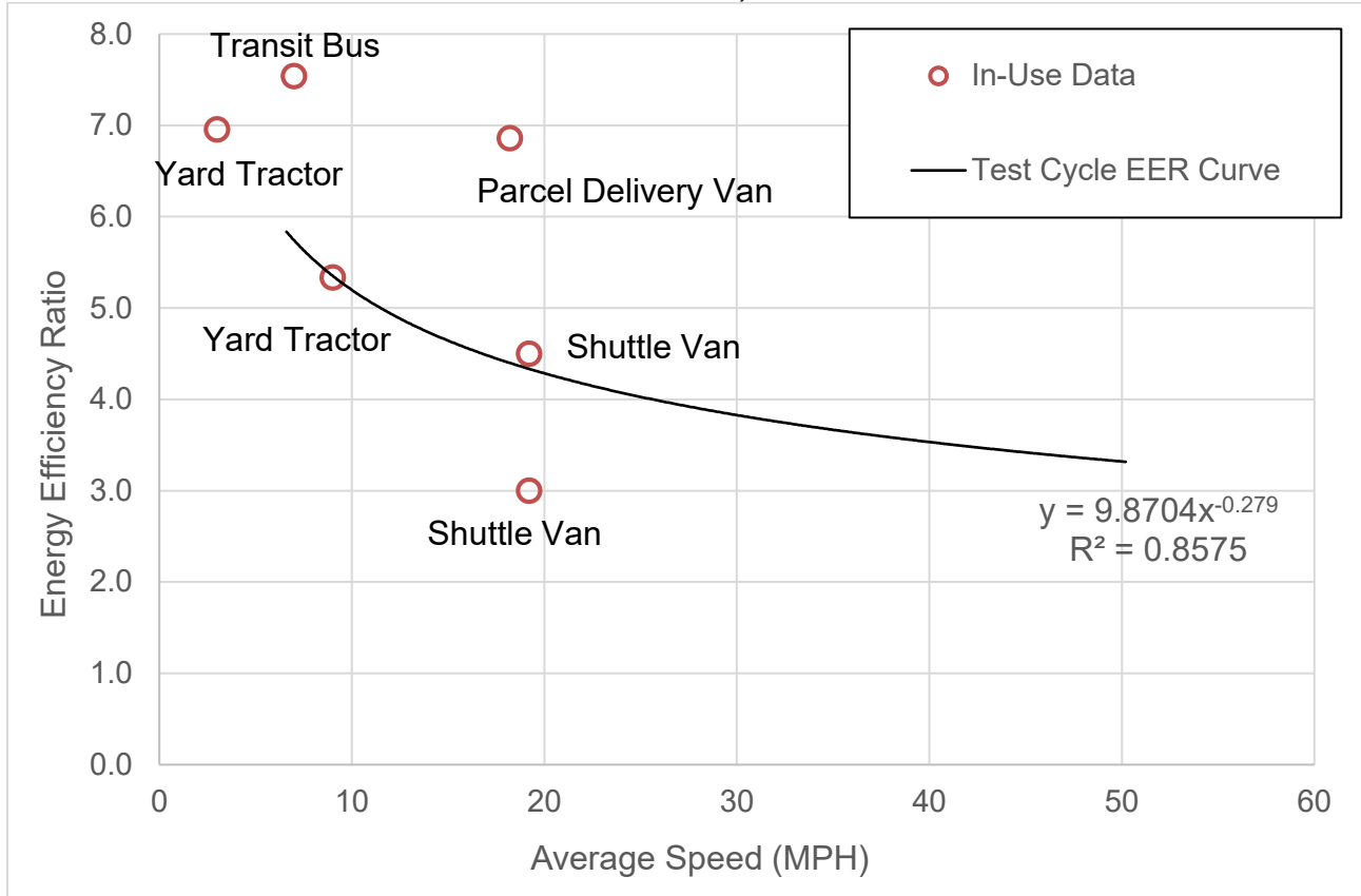
Figure 10: Vehicle Energy Efficiency Ratio at Different Average Speeds (Test Cycle and In-Use)
