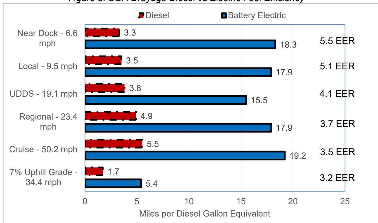
Figure 3: UCR Drayage Diesel vs Electric Fuel Efficiency
