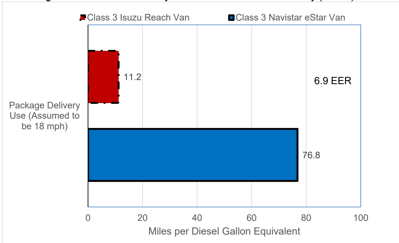
Figure 7: Parcel Van Delivery Diesel vs Electric Fuel Efficiency (In-Use)
