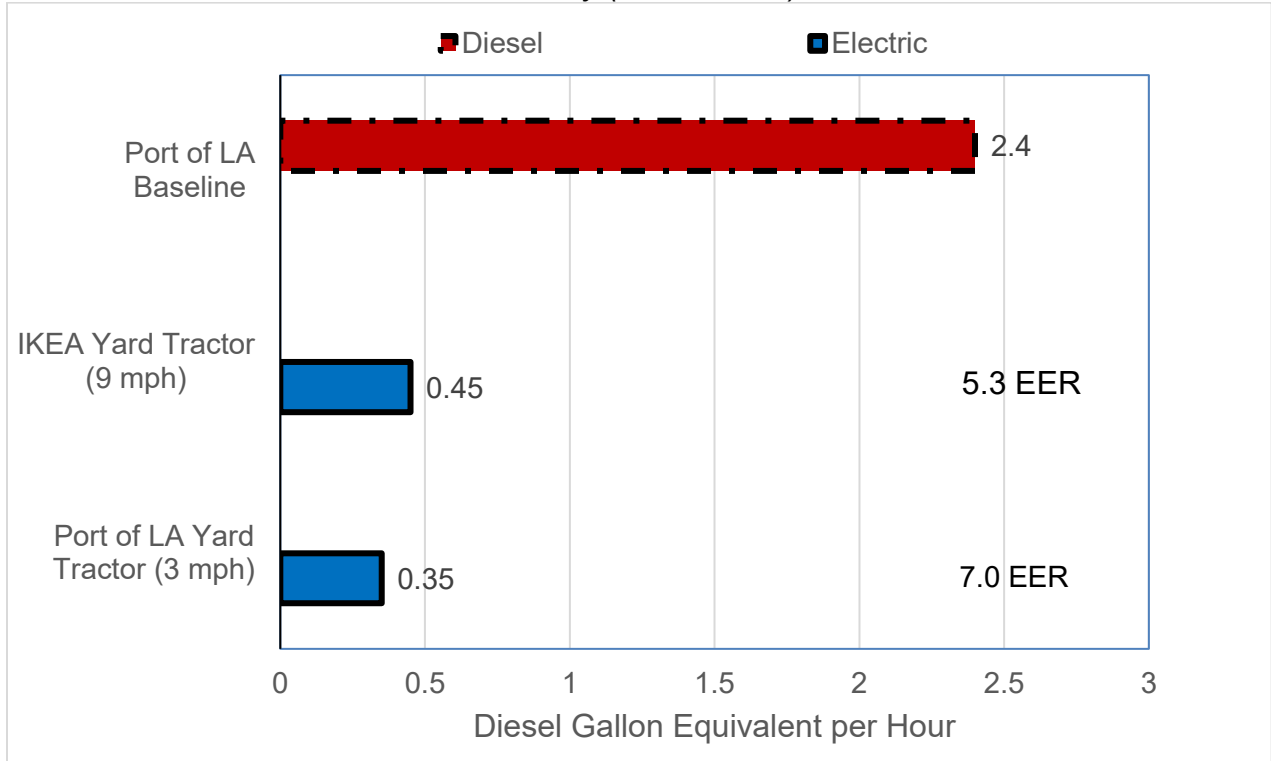
Figure 9: TransPower Yard Truck- Port and Warehouse Diesel vs Electric Fuel Efficiency (In-Use Data)
