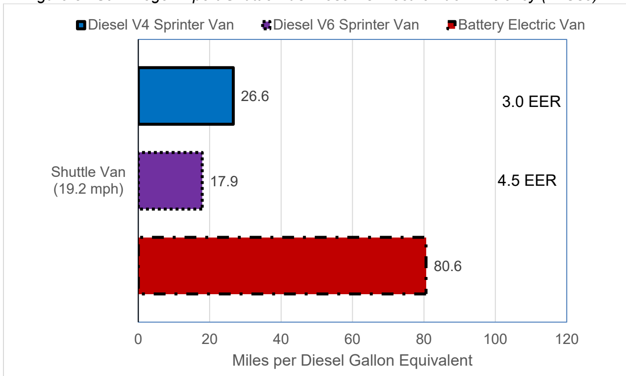
Figure 8: San Diego Airport Shuttle Bus Diesel vs Electric Fuel Efficiency (In-Use)
