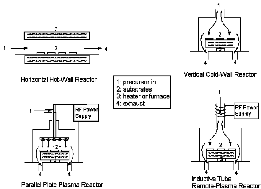
Figure III-3 Gas Movement by CVD Chamber Walls
