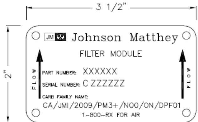
Filter Module
