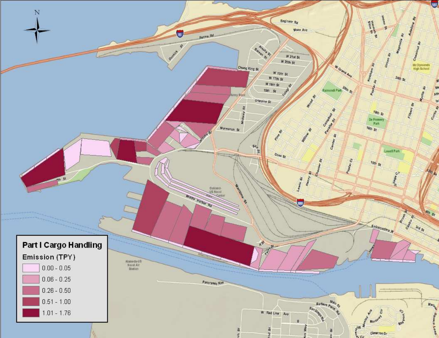
Plot E.1: Cargo Handling Emission Distribution for Part I
