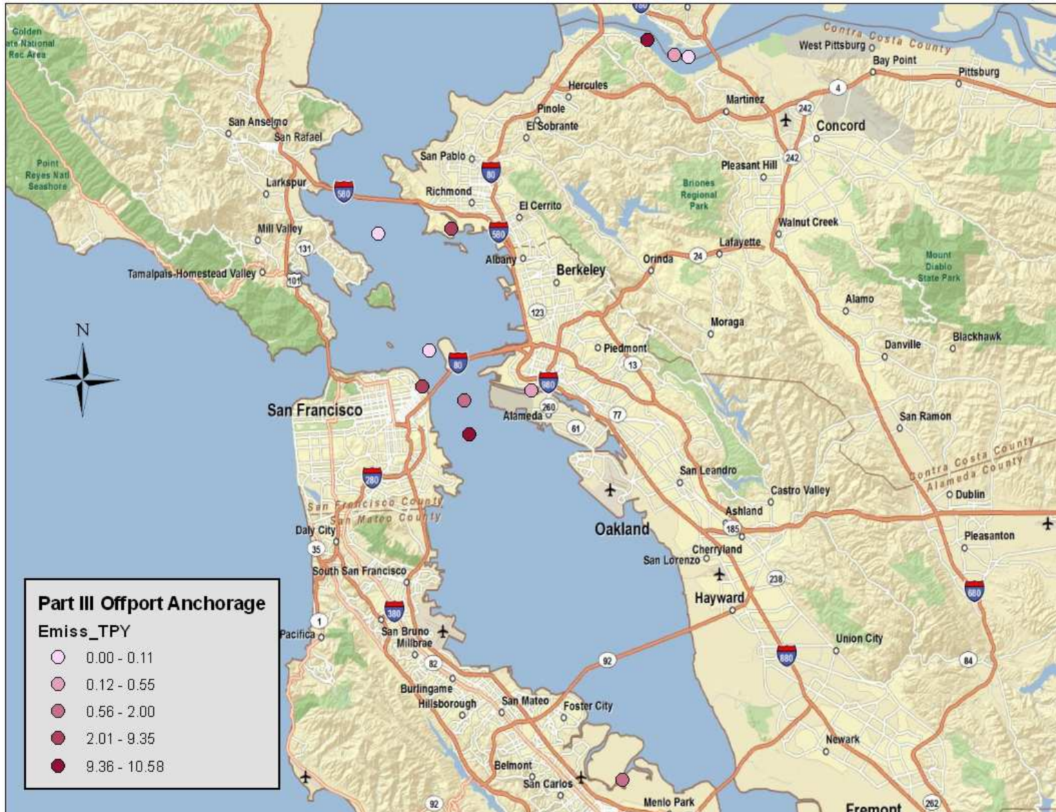
Plot E.10: Off-port Anchorage Emission Distribution for Part III
