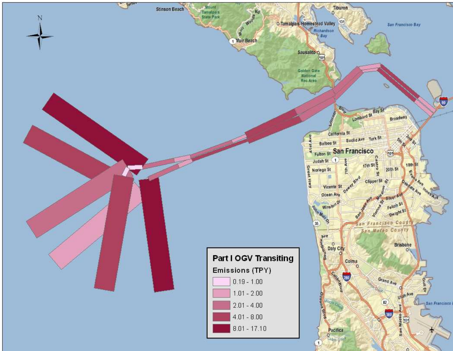
Plot E.4: Ocean Going Vessels (Transiting) Emission Distribution for Part I
