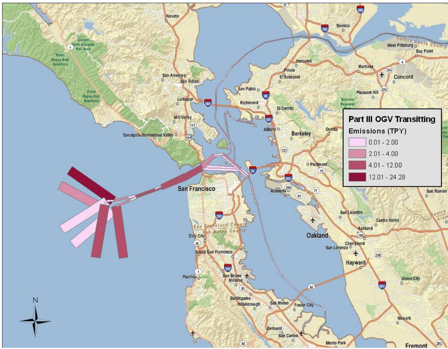
Plot E.12: Ocean Going Vessels Transiting Emission Distribution for Part III
