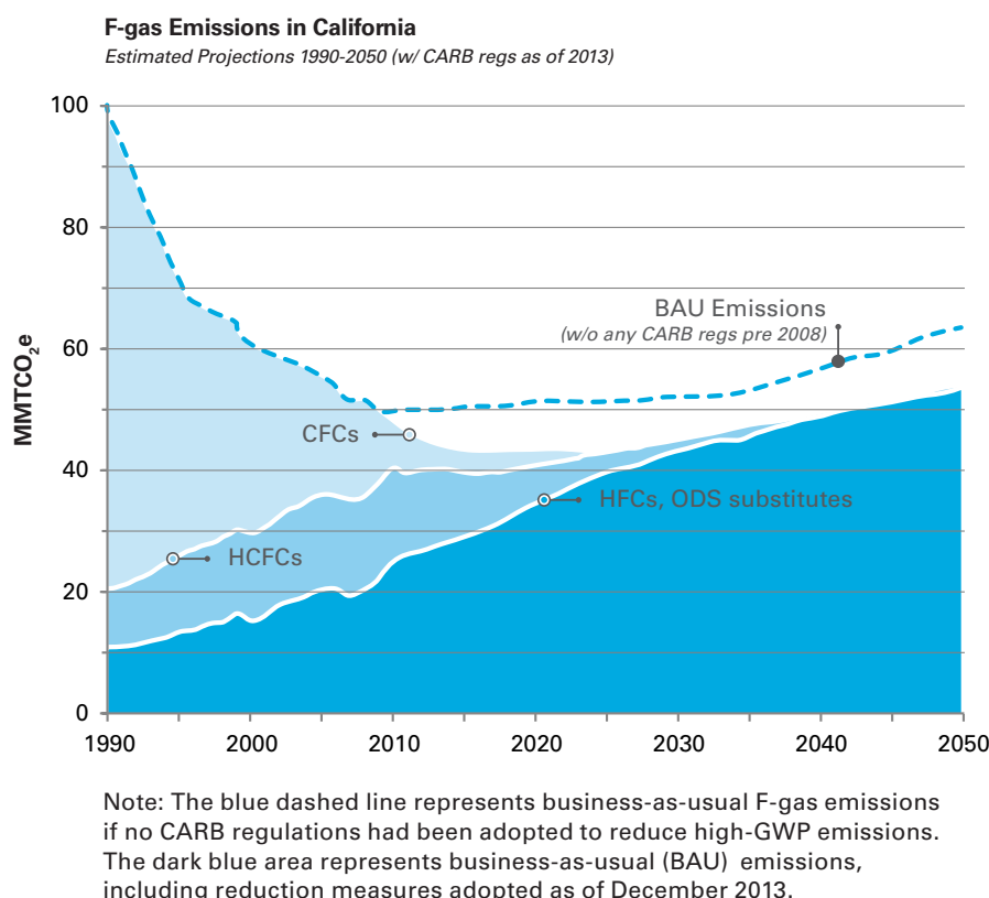
Figure 7: Fluorinated gas (F-gas) Emissions in California (1990–2050)
