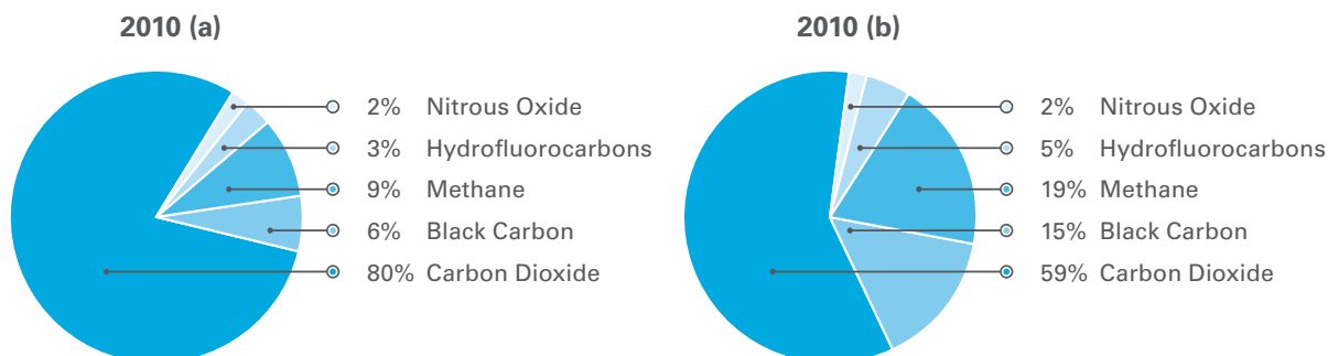
Figure 1: Carbon Dioxide Equivalent Climate Pollutant Emissions for 2010 in California Using (a) 100-year and (b) 20-year Horizon GWPs
