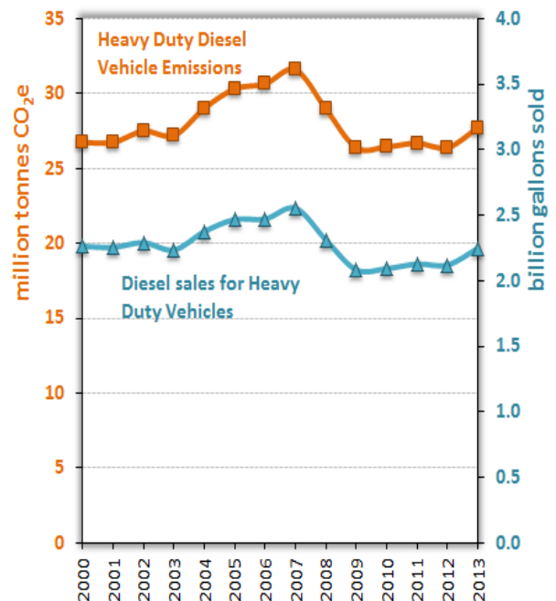
Figure 6. Transportation Diesel
