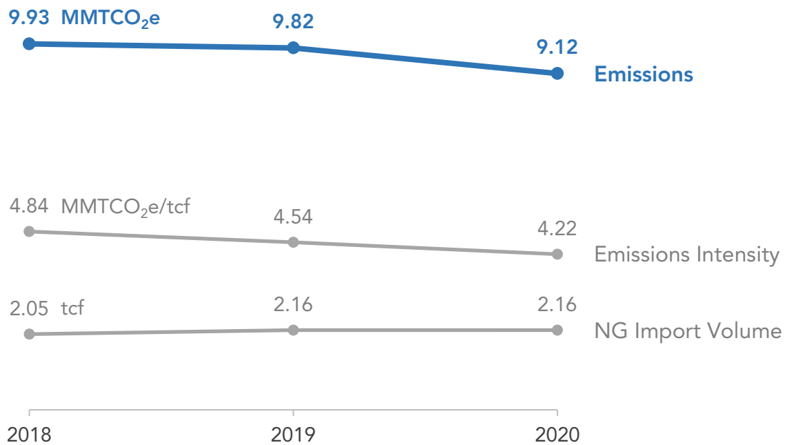
Figure 3 Trends in GHG emissions, emissions intensity, and NG import volume from 2018 to 2020 using 100-yr GWP (note, the product of the two gray lines equals the blue line, with rounding) (tcf = trillion cubic feet).
