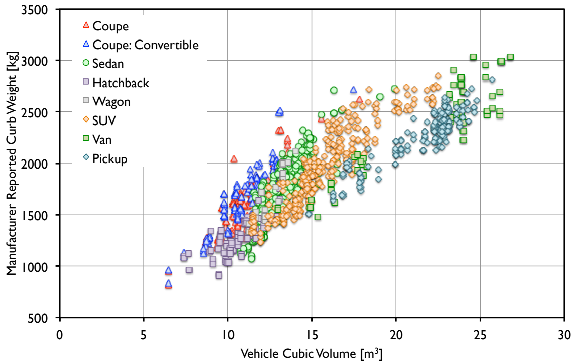
Figure 73: Manufacturer-Reported Curb Weight vs. Vehicle Cubic Volume
