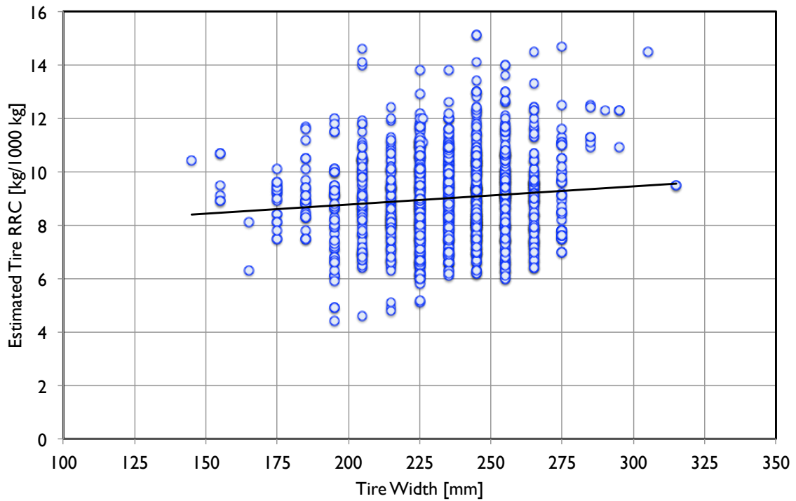
Figure 20: Estimated RRC vs. Tire Width.
