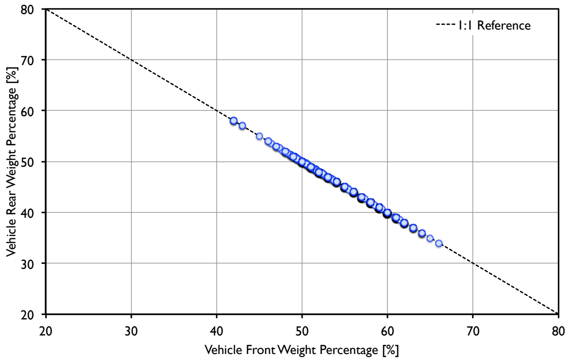
Figure 65: Rear Weight Distribution vs. Front Weight Distribution
