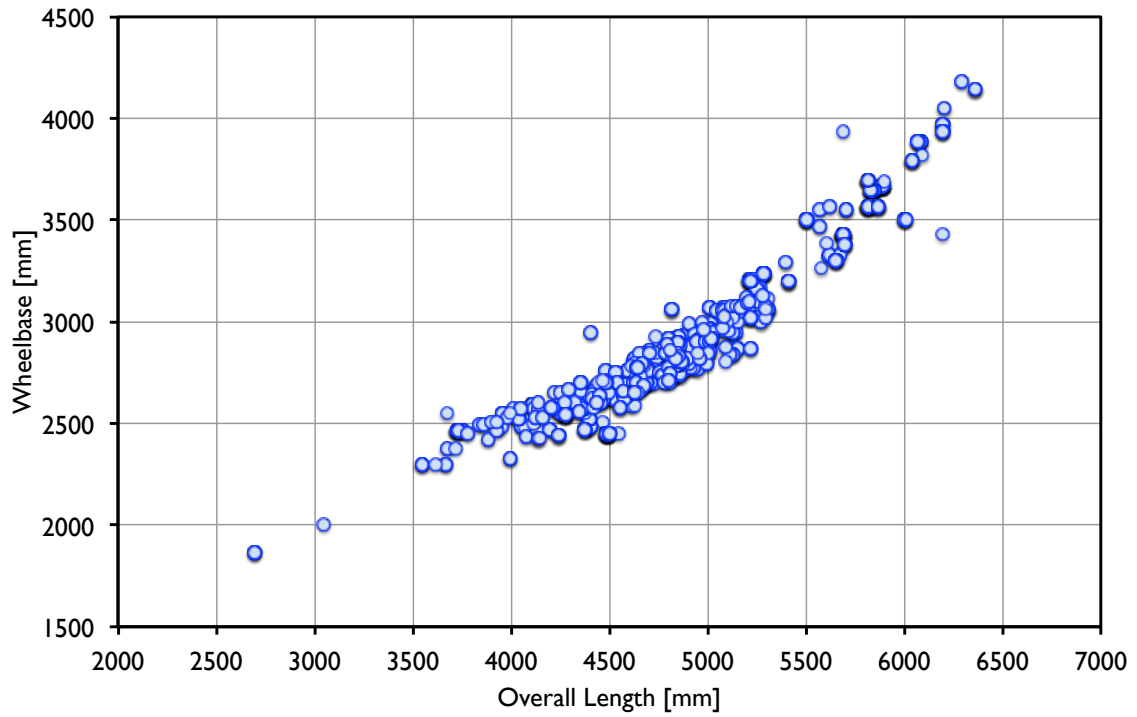
Figure 71: Wheelbase vs. Overall Length
