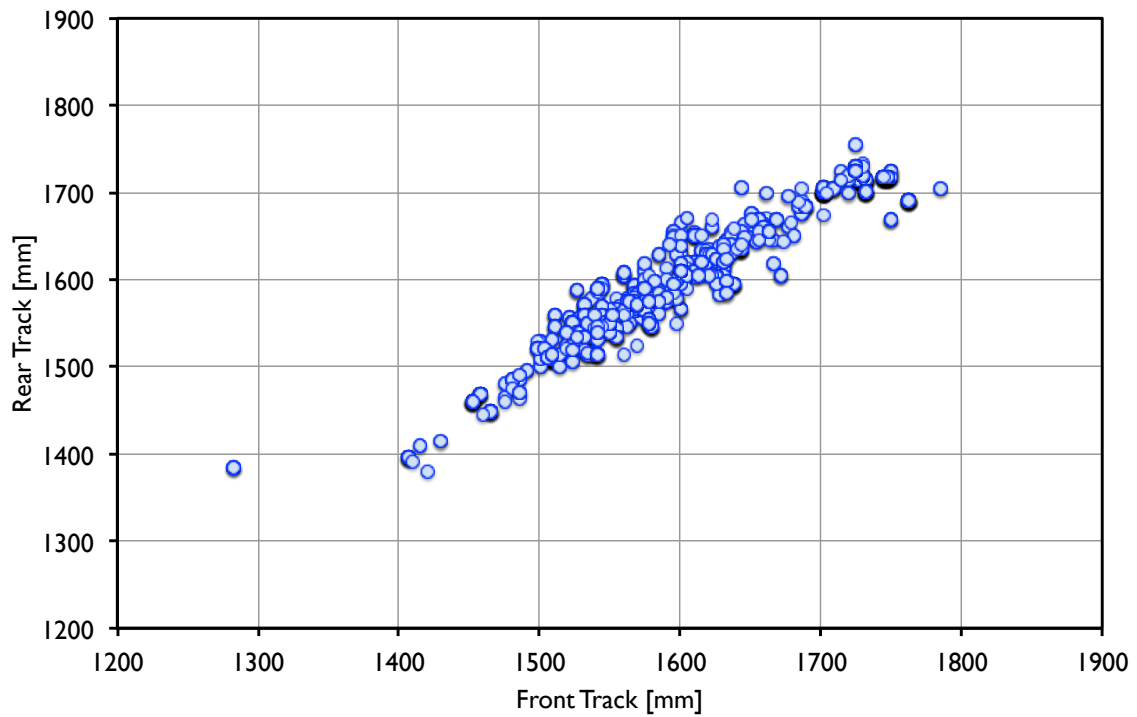
Figure 63: Rear Track vs. Front Track
