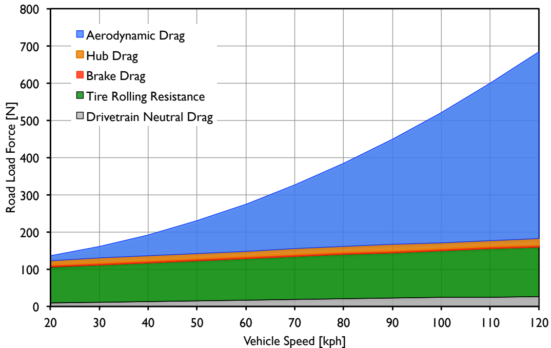
Figure 1: Road Load Force vs. Vehicle Speed.
