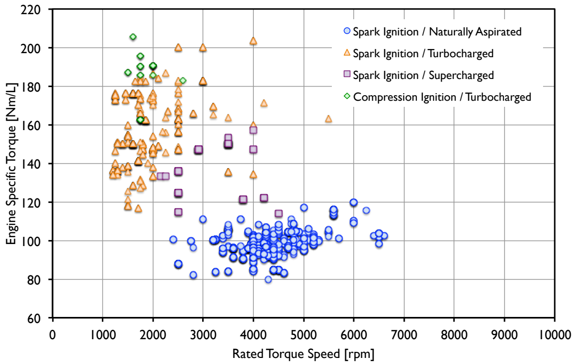
Figure 81: Engine Specific Torque vs. Rated Torque Speed
