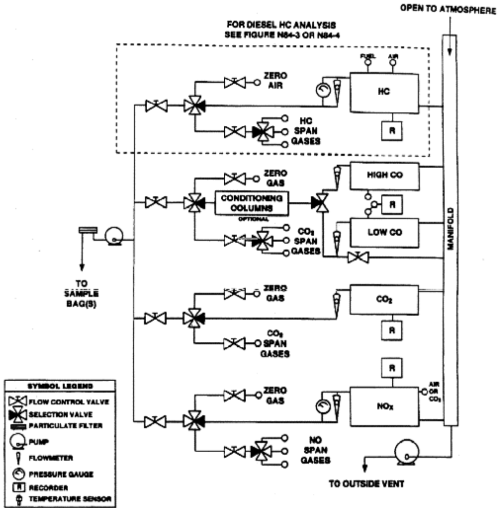
Figure 4. — Exhaust Gas Analytical System
