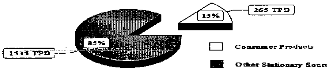
Figure IV-5 Stationary Source VOC Emissions, 1,800 Tons Per Day (TPD) in 1990
