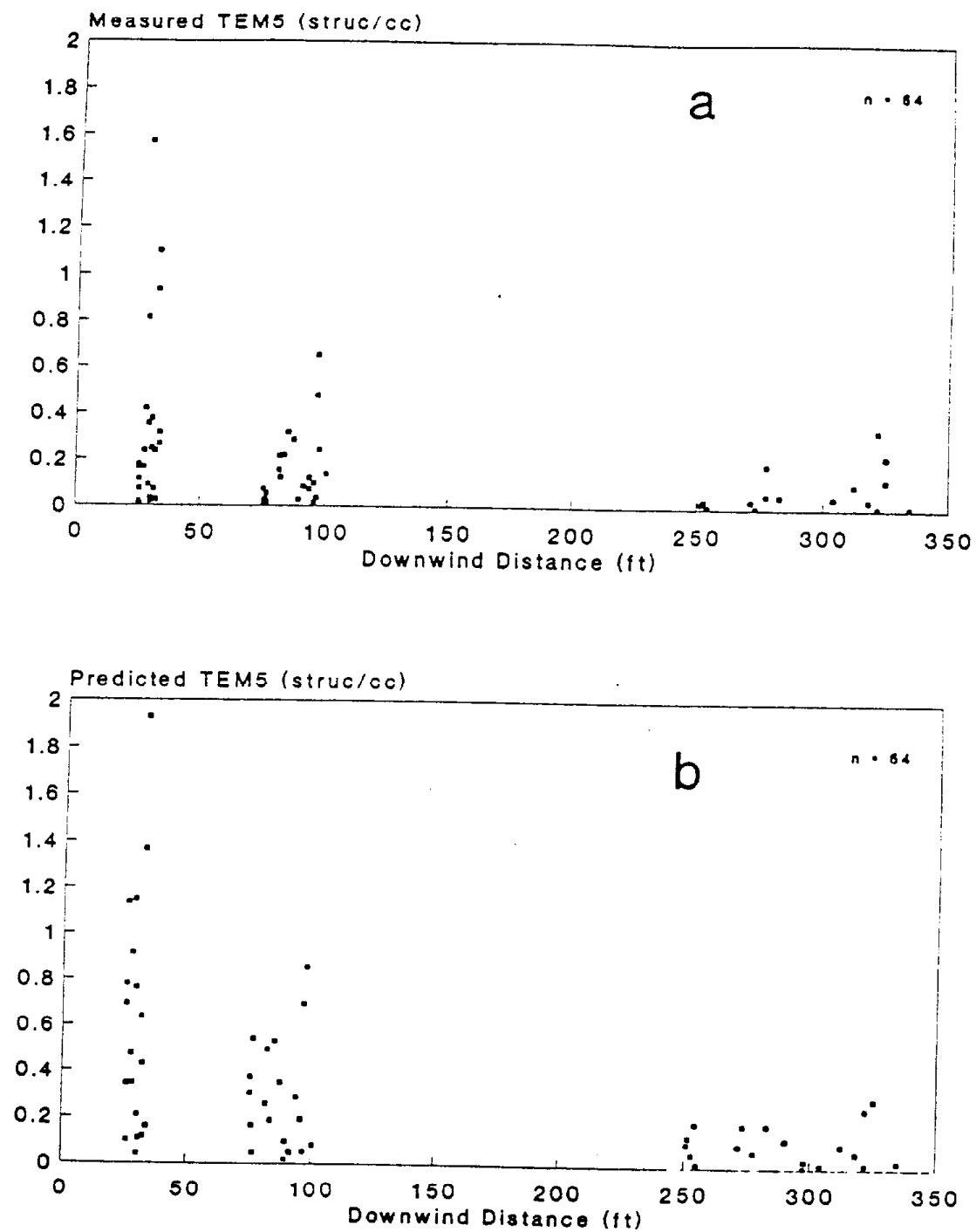
Figure 4-4. EPA Model Performance for Measured (a) vs Predicted (b) Profiles of Downwind Concentrations.
