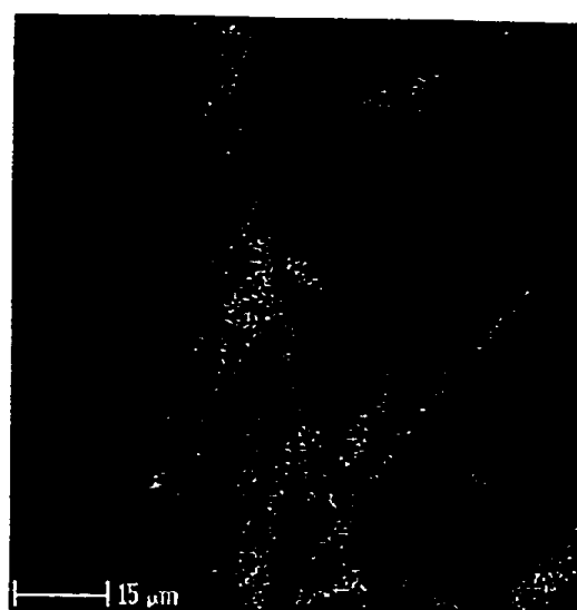
Ca-Ka (Sp2)
