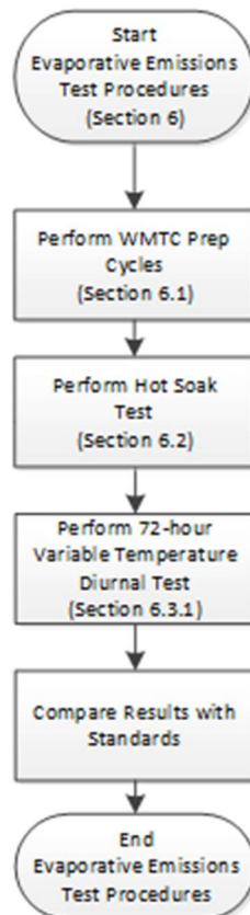
Figure 6: Evaporative Emissions Testing Flowchart
