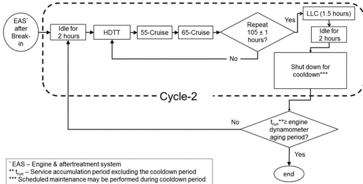
Figure CA26-43: Cycle-2 Service Accumulation Cycle
