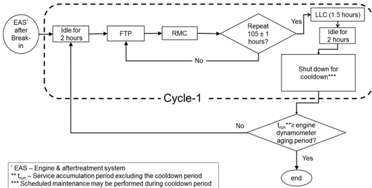
Figure CA26-32: Cycle-1 Service Accumulation Cycle
