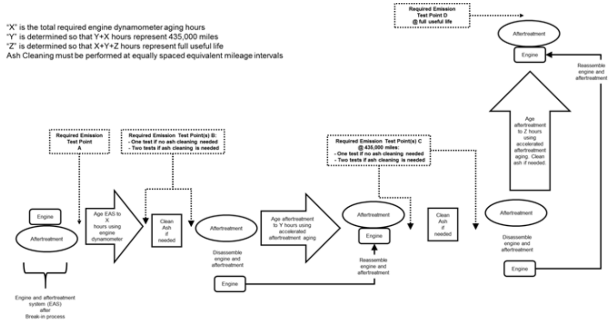
Figure CA26-54: Alternative Durability Demonstration Using Accelerated Aftertreatment Aging for 2027 and Subsequent Model Year Heavy Heavy-Duty Engines
