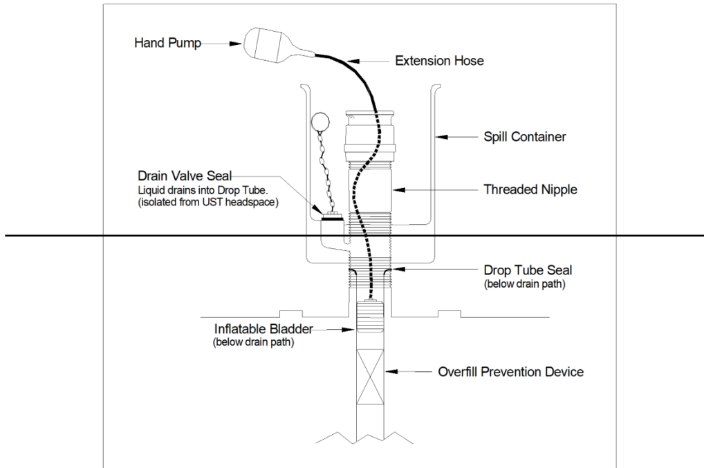
Figure 2 Typical Inflatable Bladder Installation for Direct Fill Configuration
