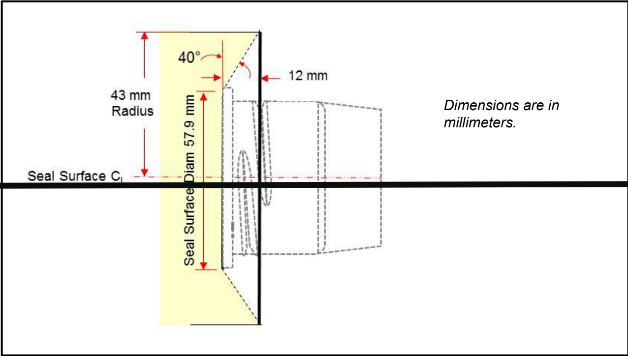
Figure 3D Fill Pipe Access Zone for Comparison to Nozzles with Spout Angles Outside of the Range Specified in Table 3-2 ( S_a of 19.5° to 26.0°)
