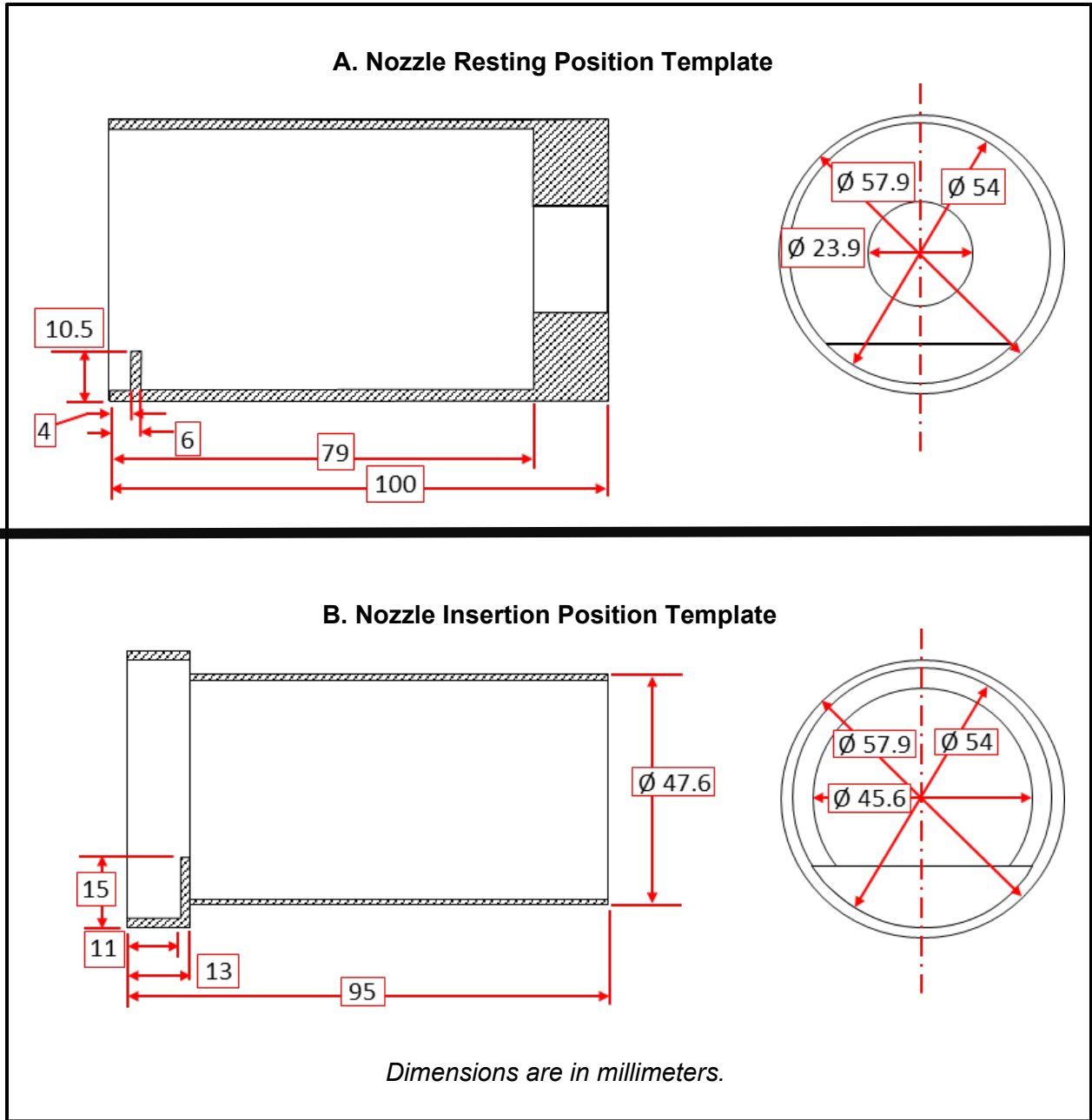
Figure 3E Fill Pipe Latching Templates for Comparison to Nozzles with Spout Angles Outside of the Range Specified in Table 3-2 ( S_a of 19.5° to 26.0°)
