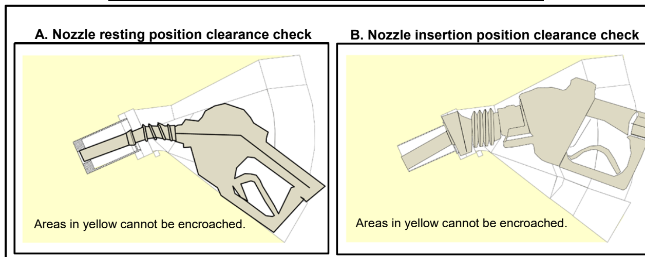
Figure 5G Nozzle Vehicle Clearance for Comparison to Nozzles with Spout Angles Outside of the Range Specified in Table 5-2 ( S\alpha of 19.5^\circ to 26.0^\circ )
