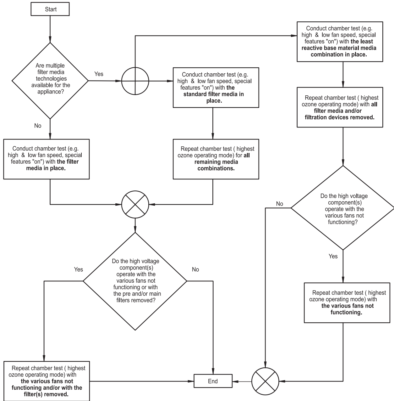
Figure 37.4.1 Filter Test Iterations Flow Chart
