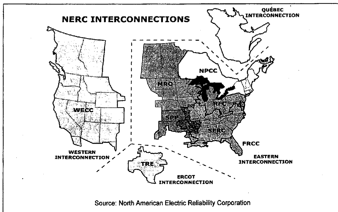
Figure III-1 North American Power Grid and Reliability Organizations
