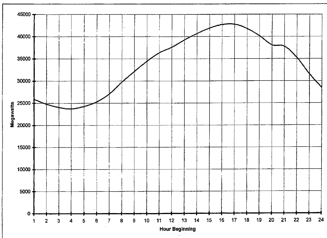
Figure III-4 CAISO System Daily Demand Curve 24 (July 14, 2009)
