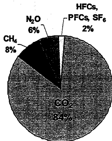
Figure 2-4: Distribution of California GHG emissions by gas in 1999, expressed in terms of \text{CO}_2 equivalent (adapted from CEC, 2002).
