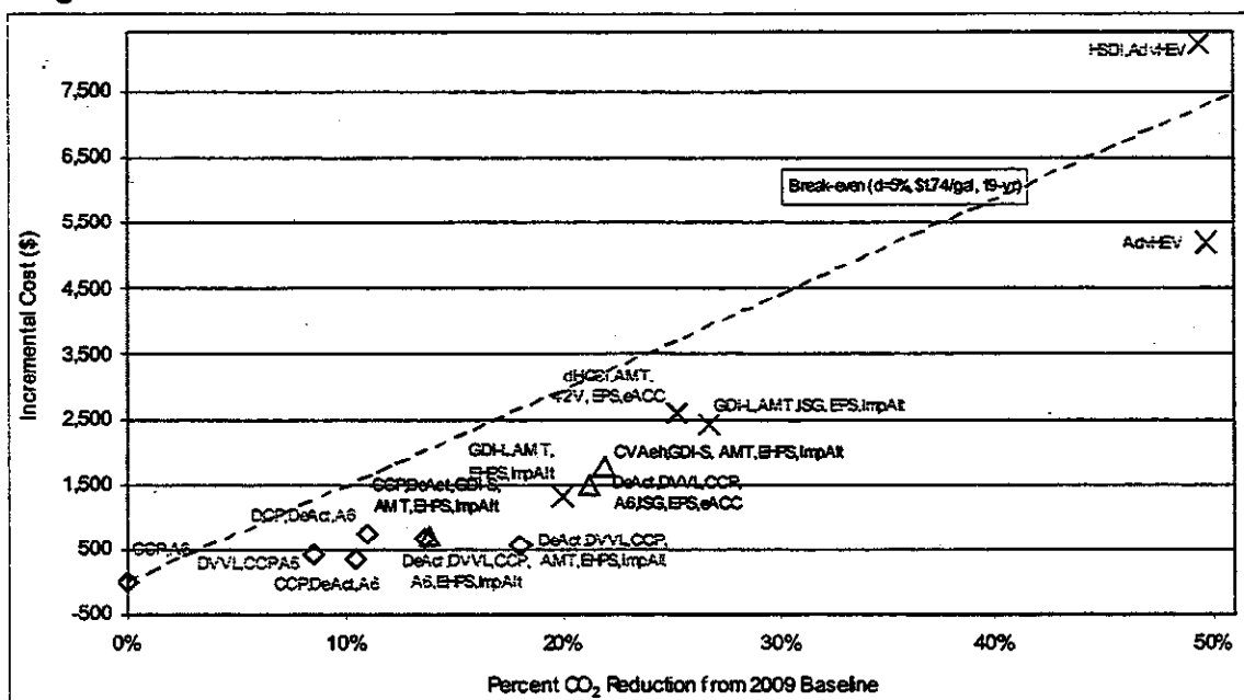
Figure 5-11. Incremental Costs for Technology Packages on 2009 Baseline Large Trucks
