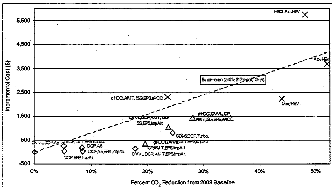
Figure 5-7. Incremental Costs for Technology Packages on 2009 Baseline Small Cars
