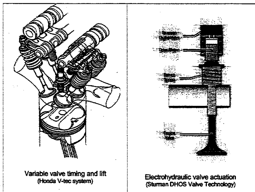
Figure 5-1: Two Variable Valve Systems
