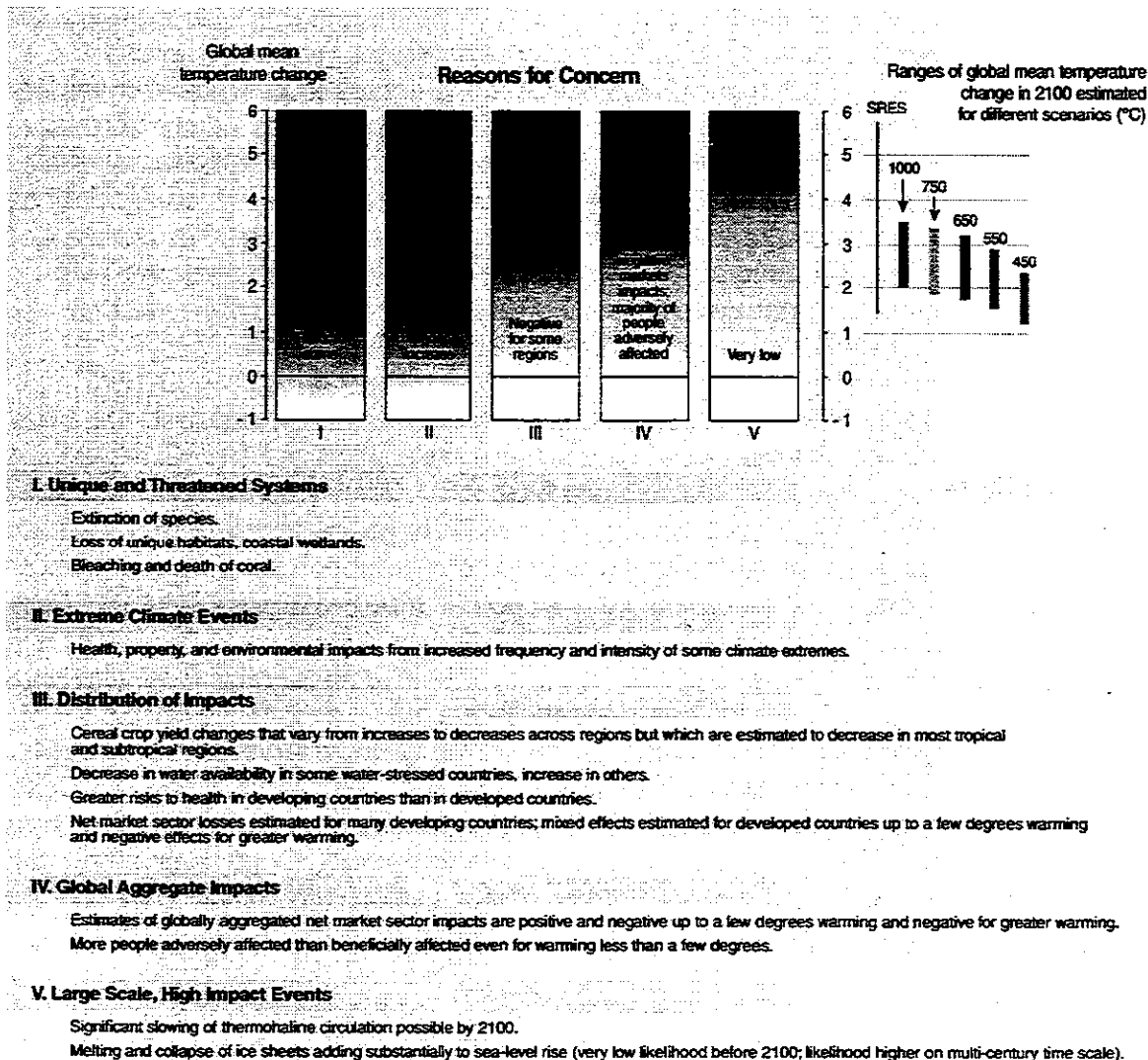
Figure 2-3. Risks of adverse impacts from climate change (source: IPCC 2001 Synthesis report).
