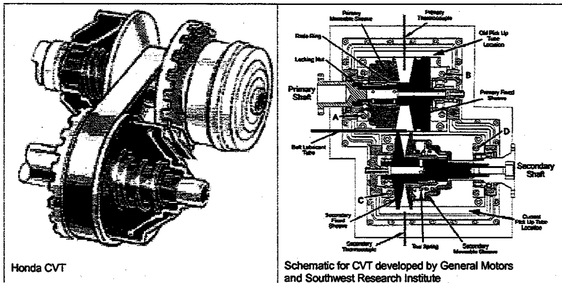
Figure 5-4: Continuously Variable Transmissions
