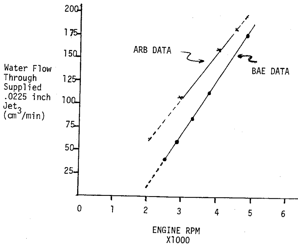
FIG 3: WATER FLOW vs. RPM UNDER BOOST CONDITIONS
