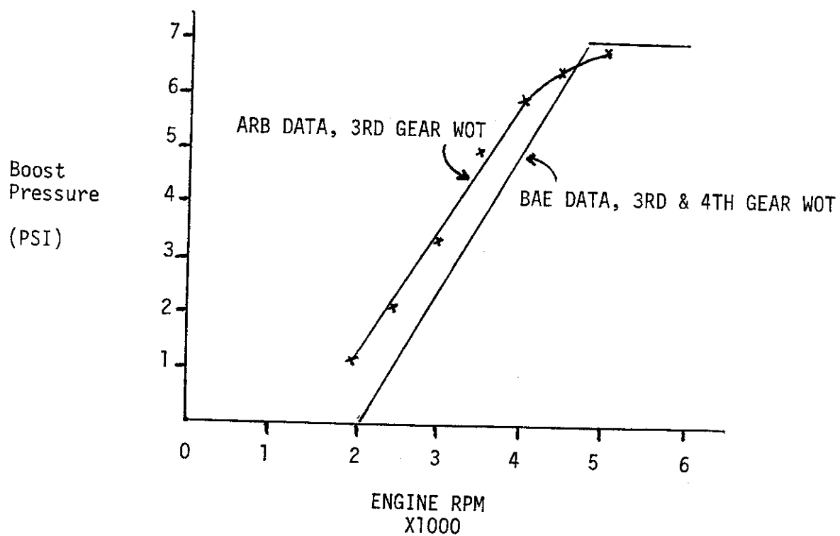
FIG 2: BOOST PRESSURE vs. RPM - TURBOCHARGED VW SCIROCCO
