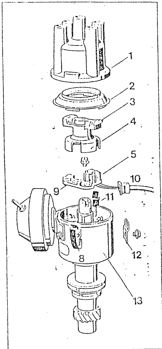
Figure 4 : Ignition distributor with Hall generator
