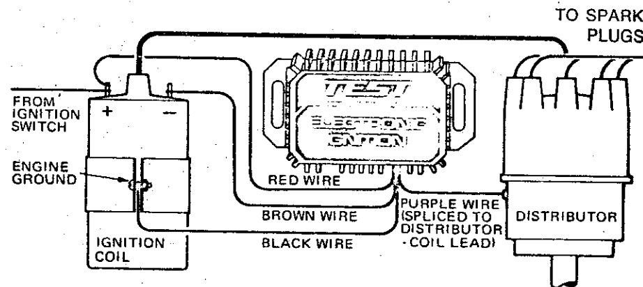
Figure 1 — WIRING DIAGRAM
