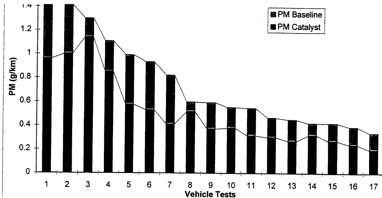
Figure 5: PM Emissions over all Chassis Test Cycles
