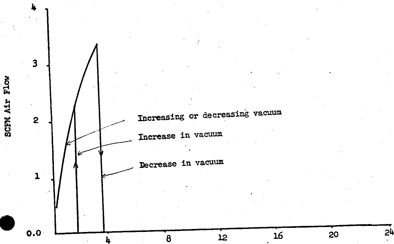
Manifold Vacuum in. of Hg Figure 2 - Second G.R. Valve
