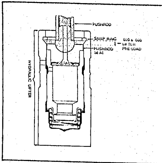
FIG. 11—Lifter preload is the distance between the pushrod seat in the lifter and the snap ring, when the lifter is on the heel of the cam and the valve is closed.
