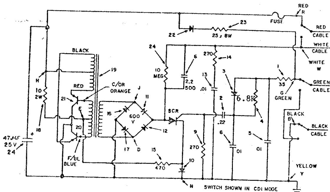
TIGER SST - SCHEMATIC DIAGRAM
