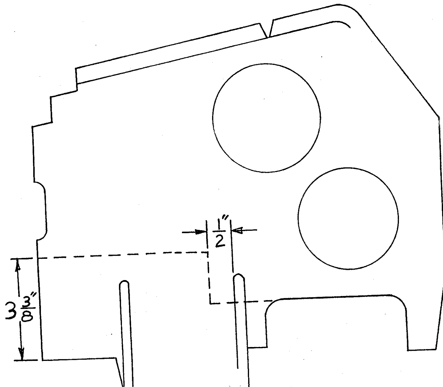
FIGURE 7 CUT LEFT PLASTIC COVER AS SHOWN. CUT ON DOTTED LINES ONLY.
