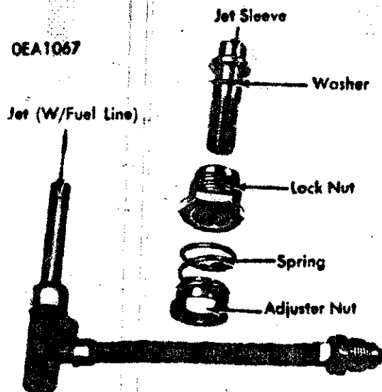
JET DISASSEMBLY (LATE MODELS)
