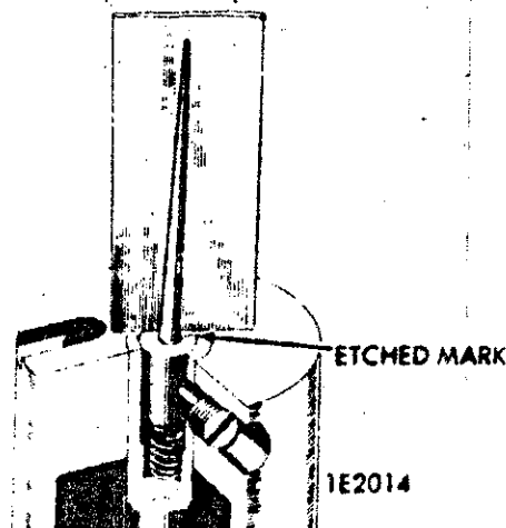
METERING NEEDLE ADJUSTMENT
