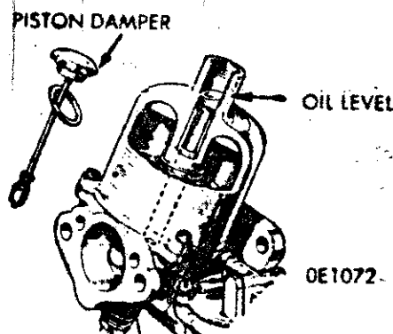
0E1072 CARBURETOR LUBRICATION
