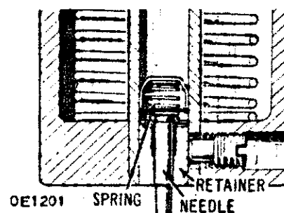
SPRING-LOADED NEEDLE
