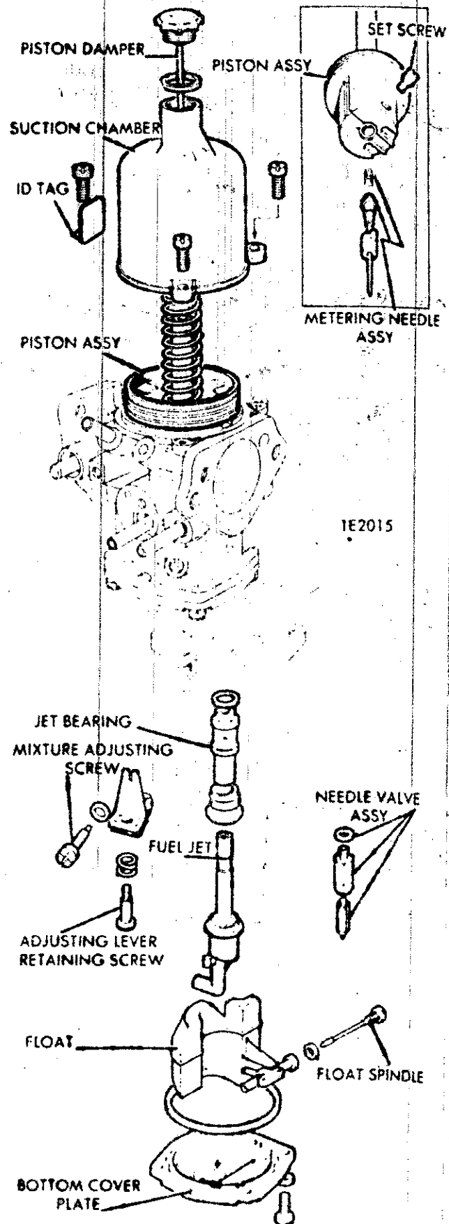
S.U. HIF6 CARBURETOR DISASSEMBLY
