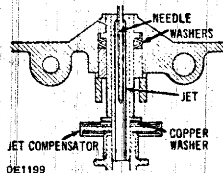
JET COMPENSATOR - TYPE I
