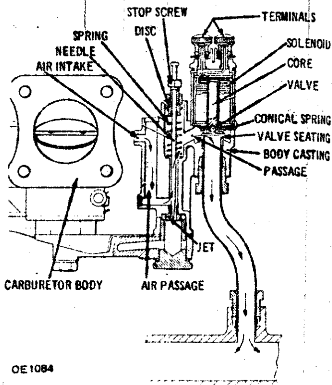
AUXILIARY ENRICHMENT CARBURETOR
