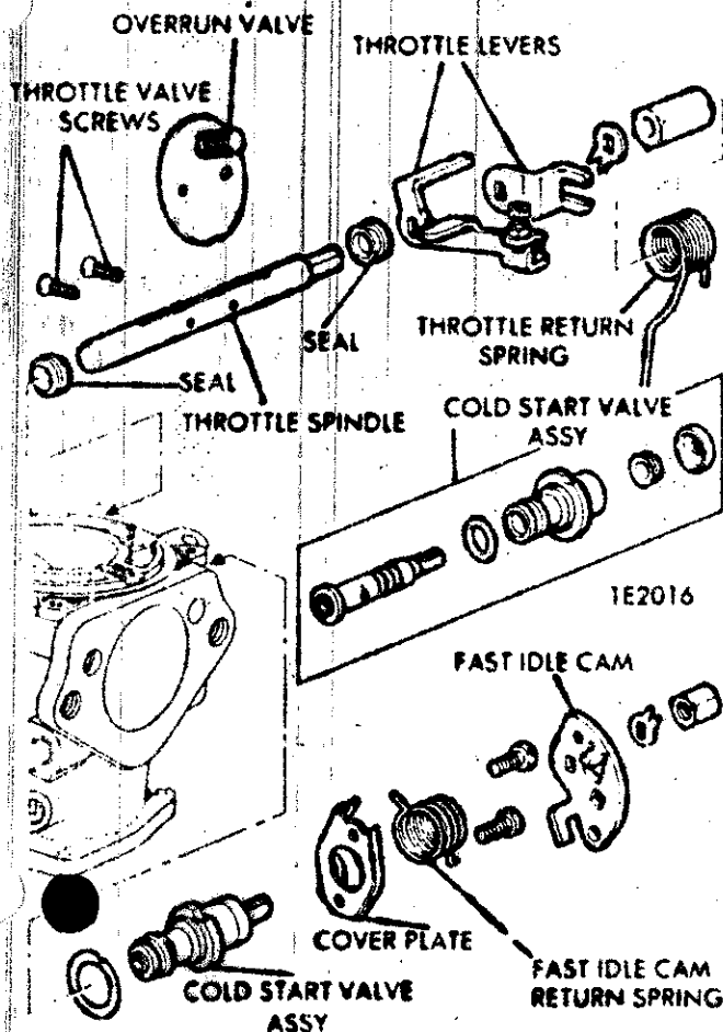
S.U. HIF6 CARBURETOR DISASSEMBLY
