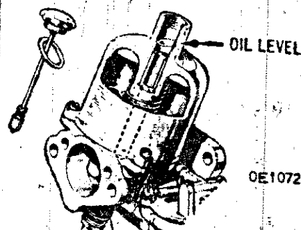
CARBURETOR LUBRICATION
