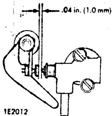
HOT START VALVE ADJUSTMENT
