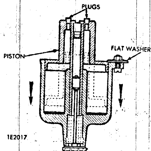
1E2017 AIR VALVE TIMING CHECK
