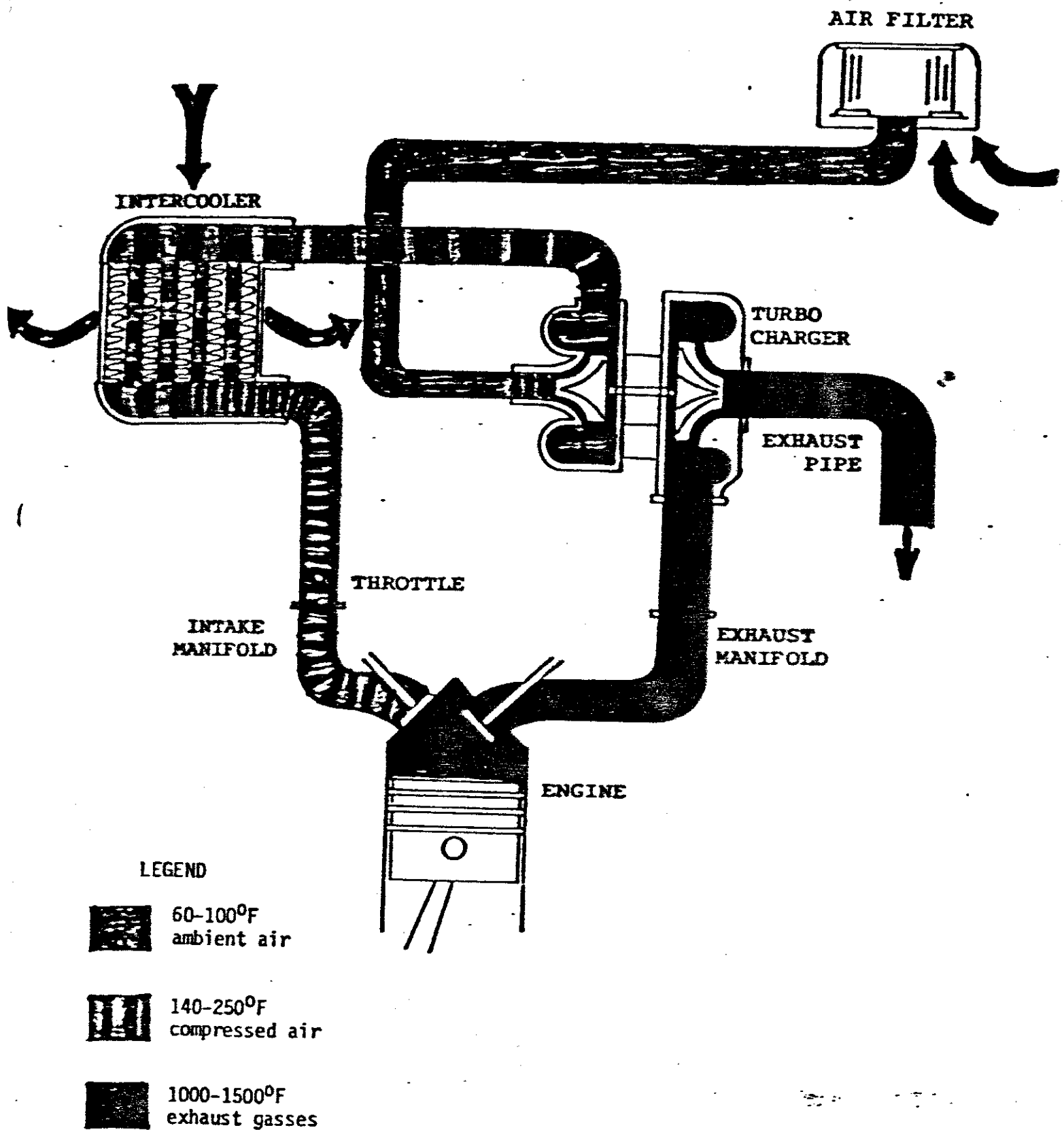
Drawing 1 Typical Installation of a 'U' Type Intercooler
