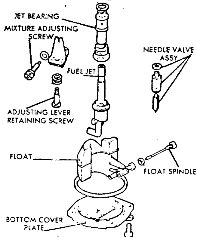
S.U. HIF CARBURETOR DISASSEMBLY
