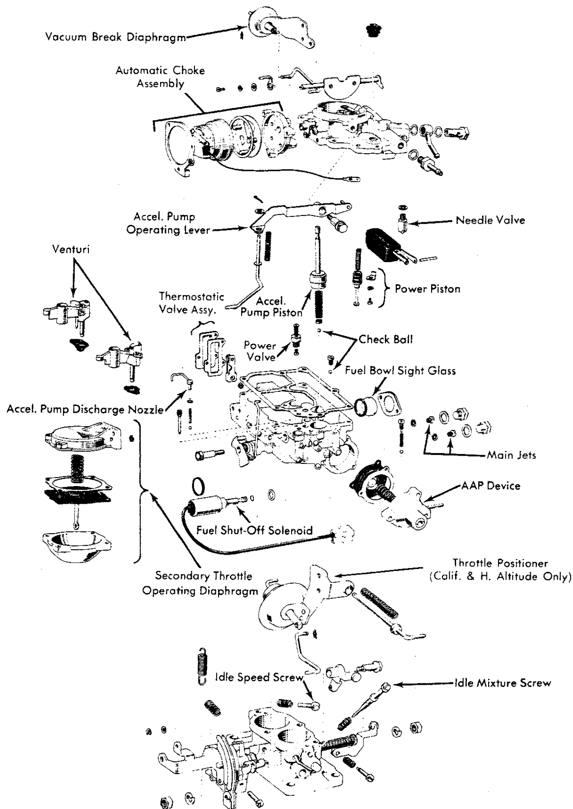
Fig. 11 Carburetor Assembly for Toyota 2T-C Engine
